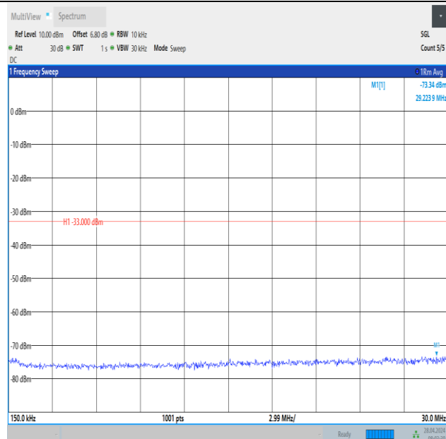
Band2_20MHz_16QAM_18700_1RB#99_0.15~30_0.15~30
