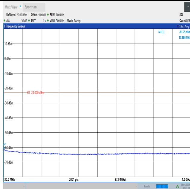
Band2_20MHz_QPSK_18700_1RB#99_30~1000_30~1000
