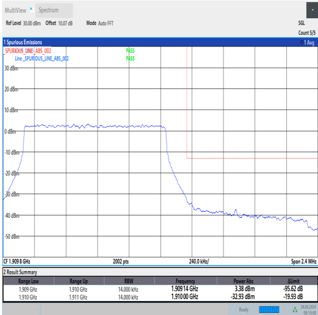
Band2_1.4MHz_QPSK_19193_6RB#0
