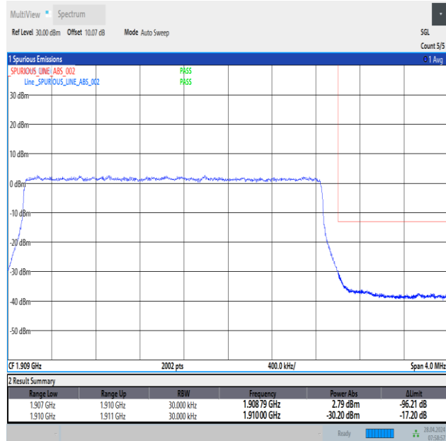
Band2_3MHz_QPSK_19185_15RB#0
