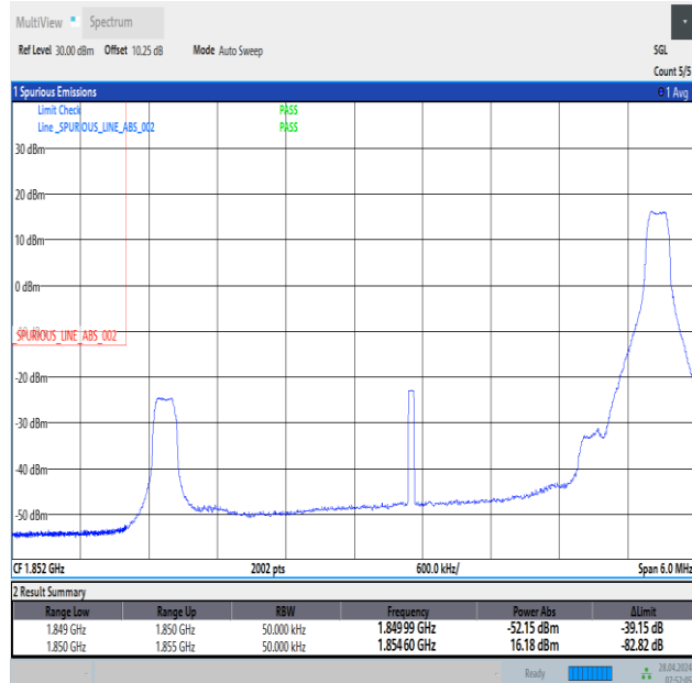
Band2_5MHz_QPSK_18625_1RB#24
