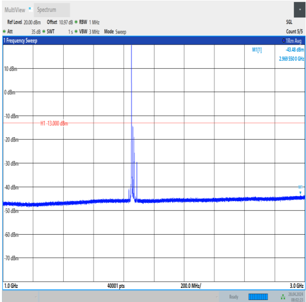
Band2_20MHz_16QAM_18700_1RB#0_1000~3000_1000~3000
