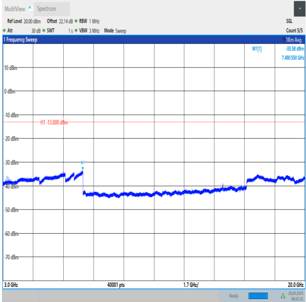
Band2_20MHz_16QAM_18700_1RB#0_3000~20000_3000~20000
