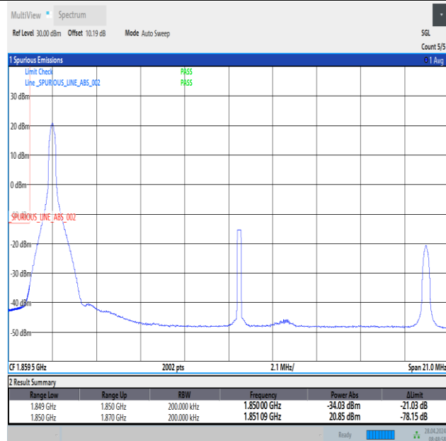
Band2_20MHz_16QAM_18700_1RB#0
