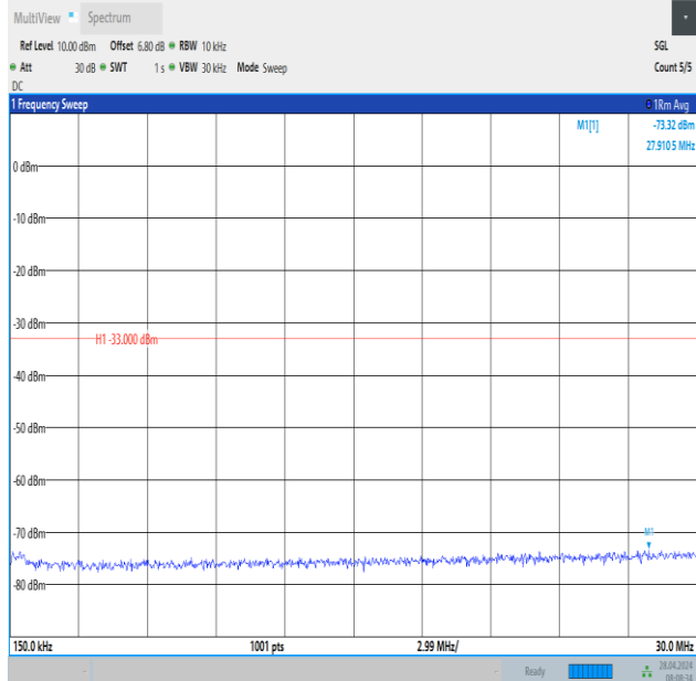
Band2_20MHz_QPSK_19100_1RB#0_0.15~30_0.15~30
