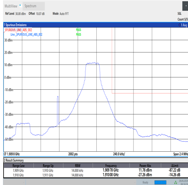
Band2_1.4MHz_QPSK_19193_1RB#5
