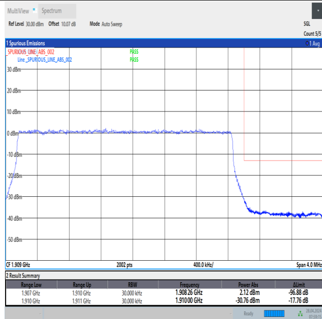
Band2_3MHz_16QAM_19185_15RB#0
