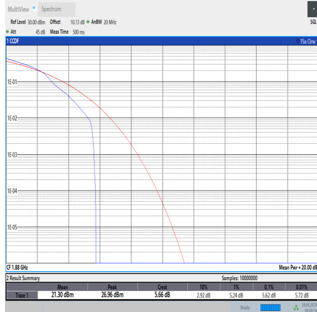
Band2-15MHz-16QAM-18900-1RB#0-PASS
