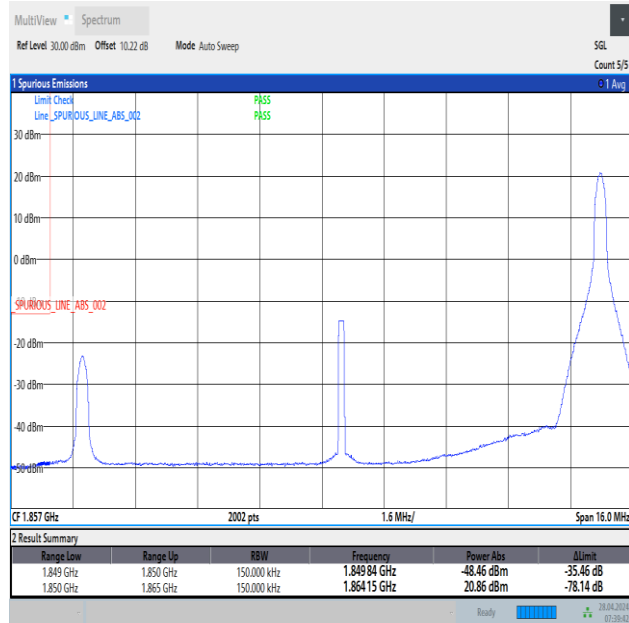
Band2_15MHz_QPSK_18675_1RB#74
