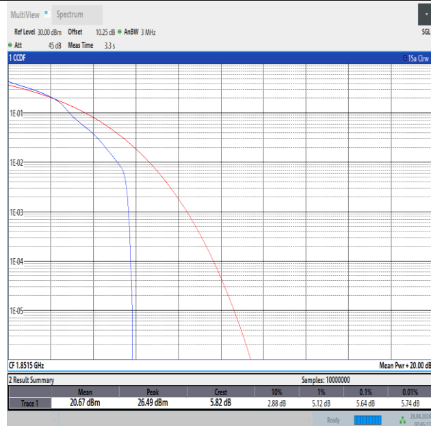
Band2-3MHz-16QAM-18615-1RB#0-PASS
