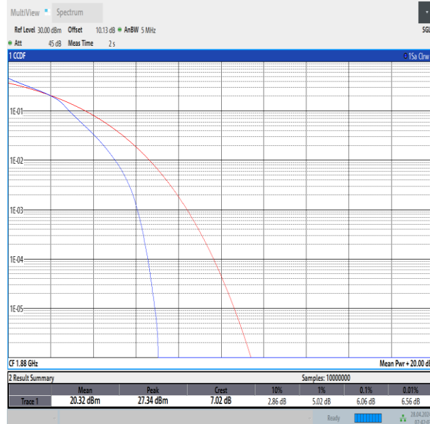
Band2-5MHz-16QAM-18900-25RB#0-PASS
