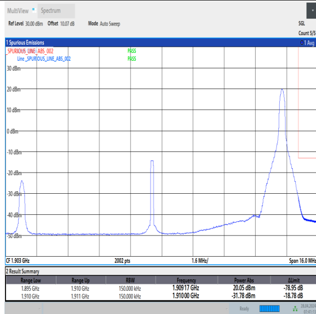
Band2_15MHz_16QAM_19125_1RB#74
