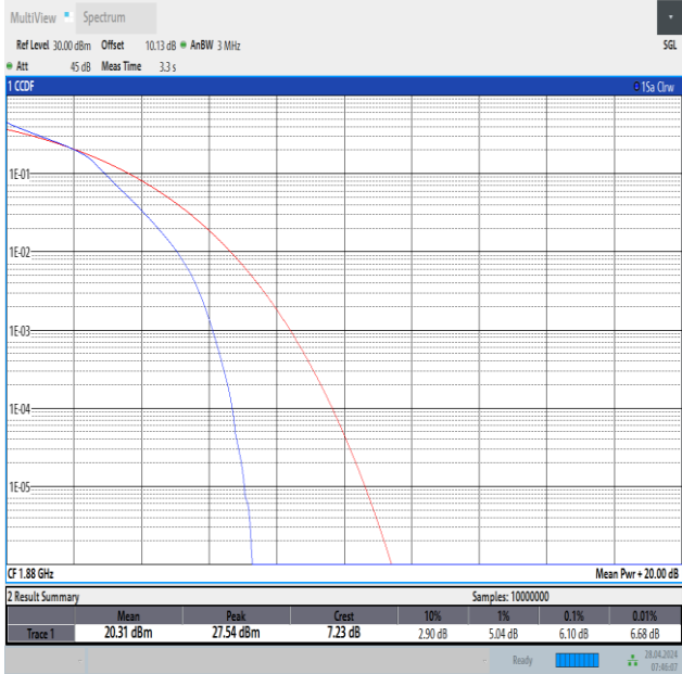
Band2-3MHz-16QAM-18900-15RB#0-PASS
