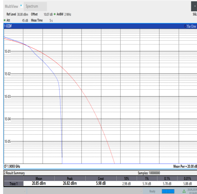
Band2-1.4MHz-16QAM-19193-1RB#0-PASS
