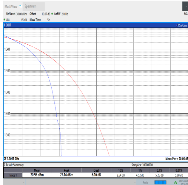
Band2-1.4MHz-QPSK-19193-6RB#0-PASS
