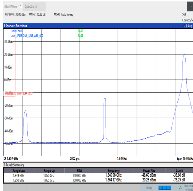
Band2_15MHz_16QAM_18675_1RB#74
