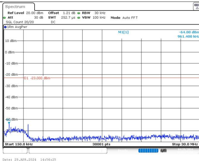
Band4-1413-2-0.15~30MHz
