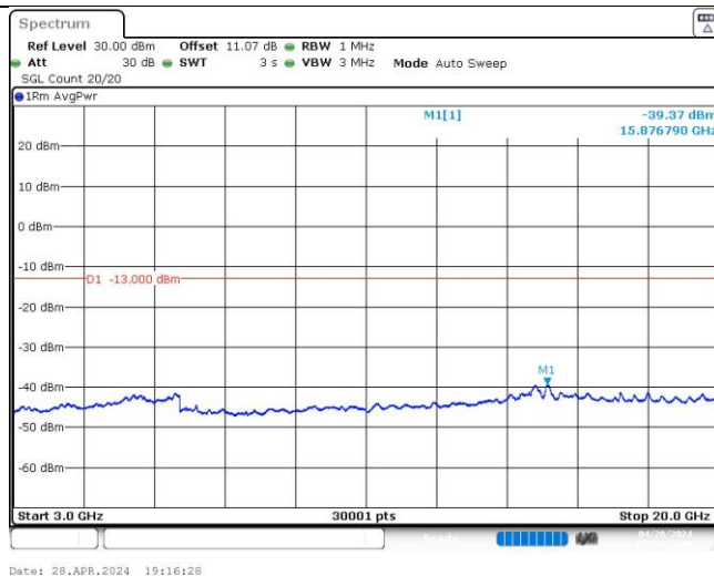
Band2-9538-4-3000~20000MHz
