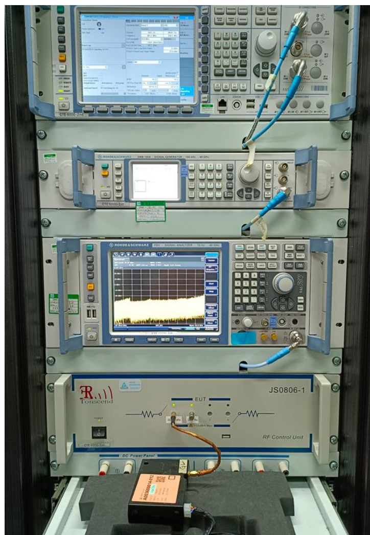
Photograph 2: Set-up photo for Conducted Measurement
