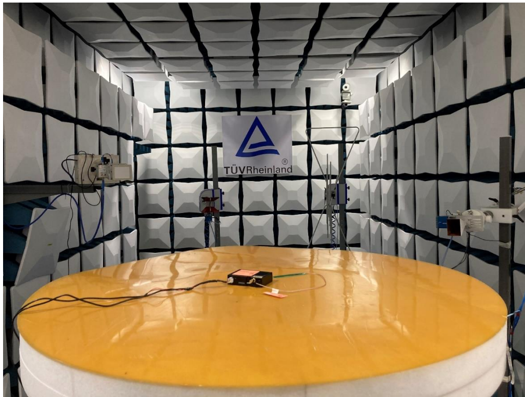
Photograph 1: Set-up photo for Radiated Spurious Emission, 30MHz - 18GHz
