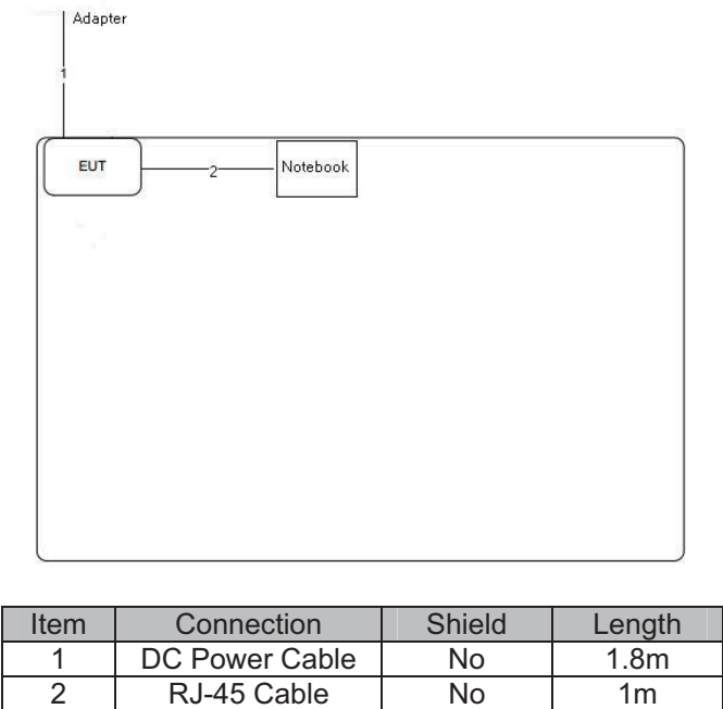
Fig. 2-1 Configuration of Tested System
