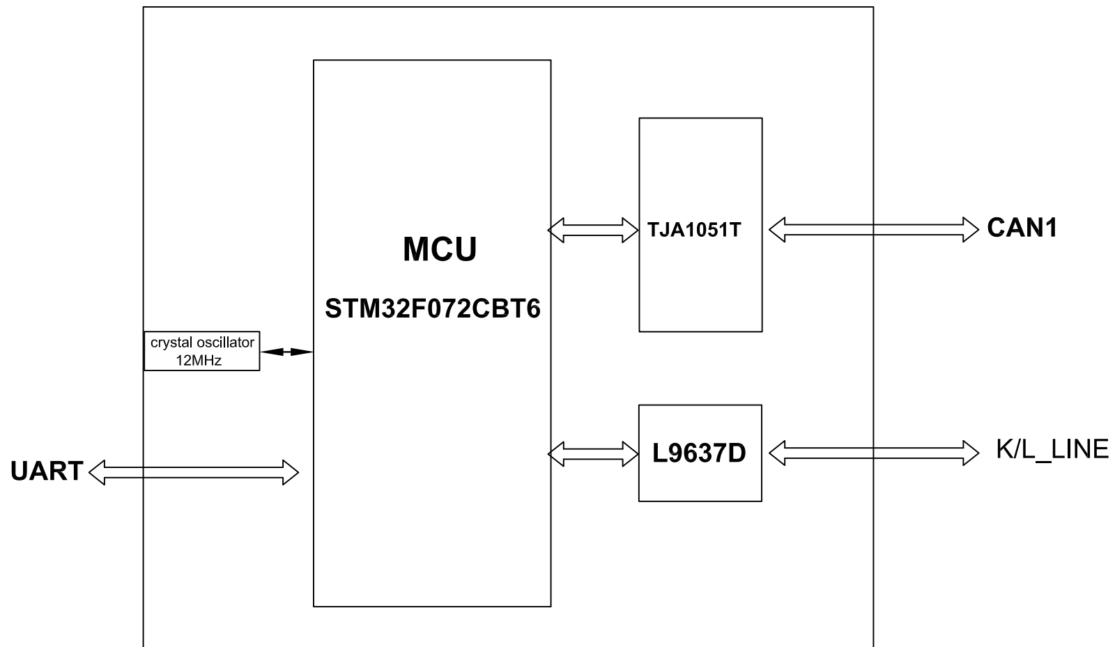
System Diagram
