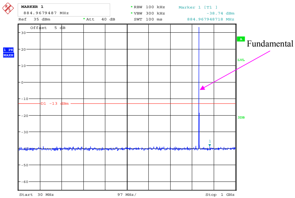
GSM850_Middle Channel
