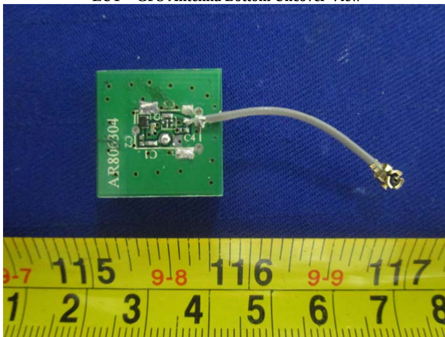
EUT – GPS Antenna Bottom Uncover View
