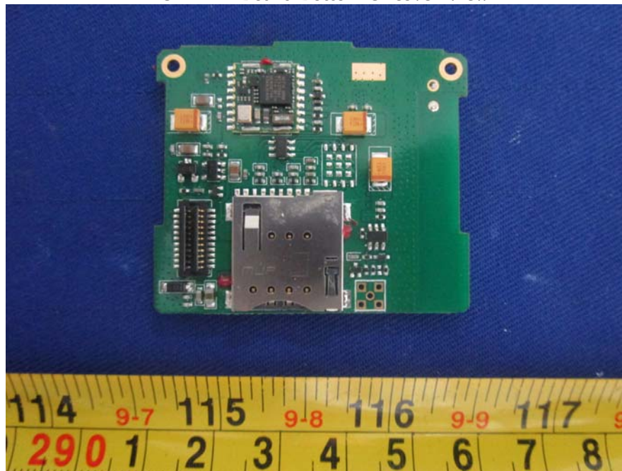
EUT – RF Board Bottom Uncover View
