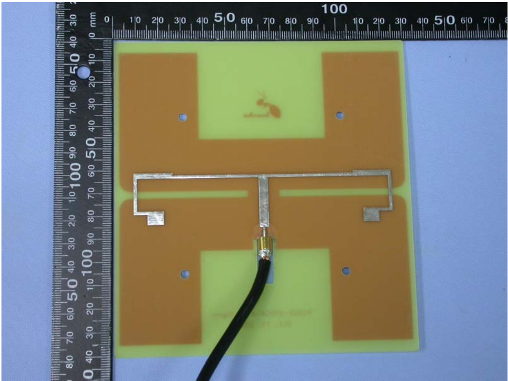
12. Rear view of PCB (A9235-A-002-NET)
