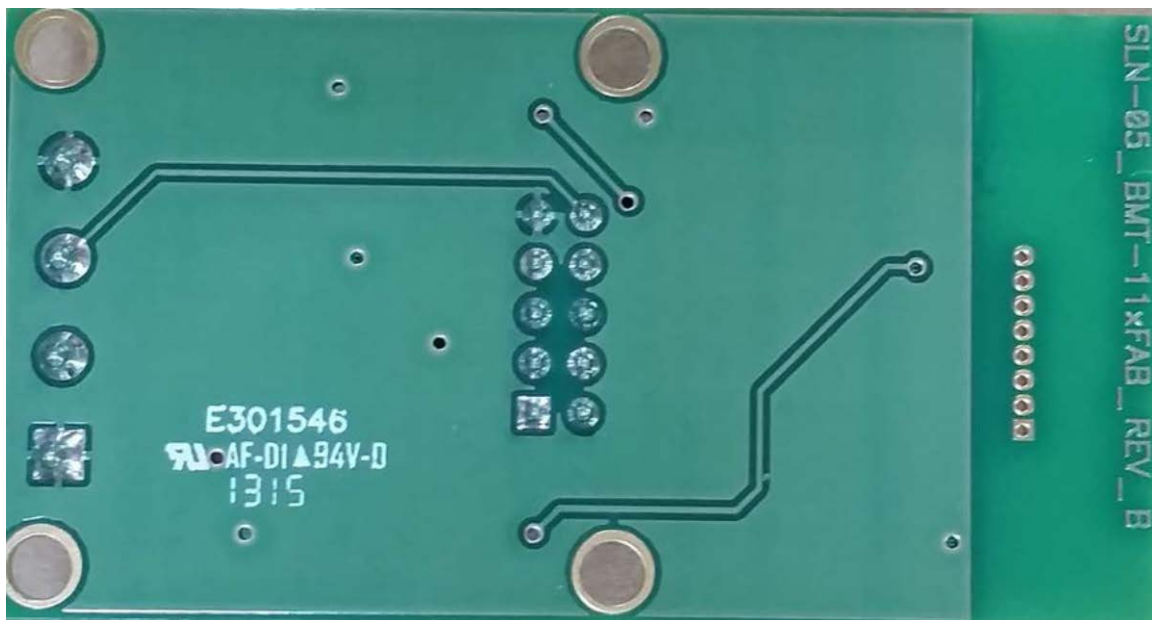
BT 2.0 Module, PCB1, Bottom View
