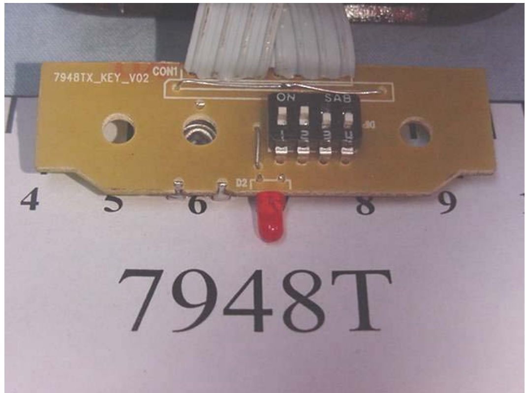
FIGURE 4 MOTION SENSOR WITH RF REMOTE (M/N: 7948T) MAIN BOARD 2 (COMPONENT SIDE)
