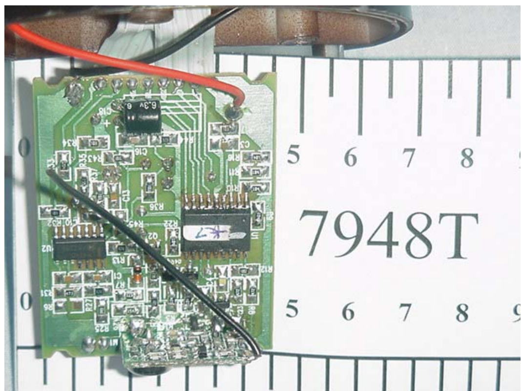
FIGURE 3 MOTION SENSOR WITH RF REMOTE (M/N: 7948T) MAIN BOARD 1 (SOLDERED SIDE)
