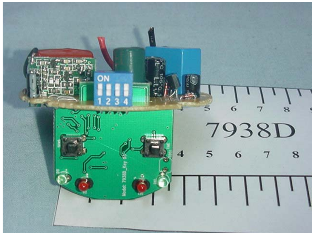
FIGURE 3 MOTION SENSOR WITH RF TRANSMITTER (M/N: 7938D) MAIN BOARD 1 (COMPONENT SIDE)
