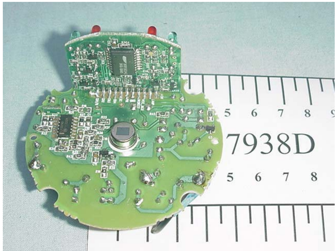
FIGURE 5 MOTION SENSOR WITH RF TRANSMITTER (M/N: 7938D) MAIN BOARD 1&2 (SOLDERED SIDE)
