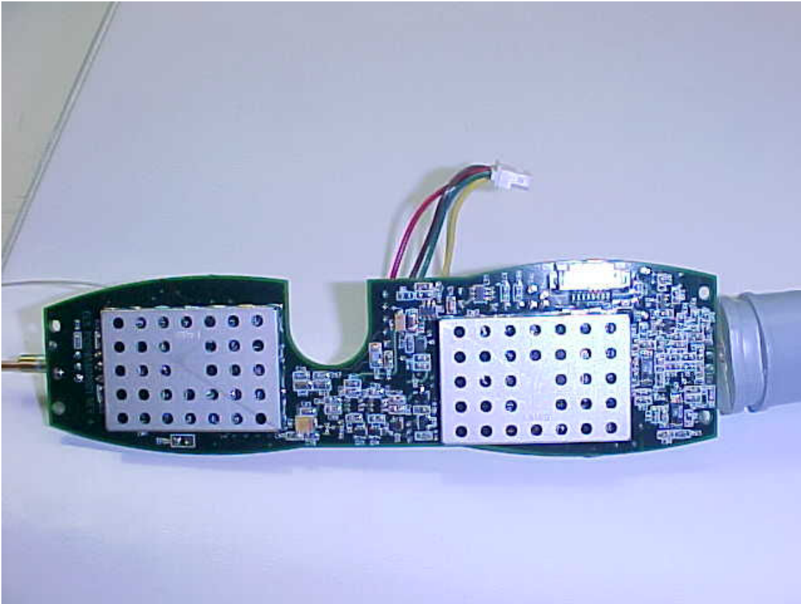
X Unit, Rear PCB Layout
