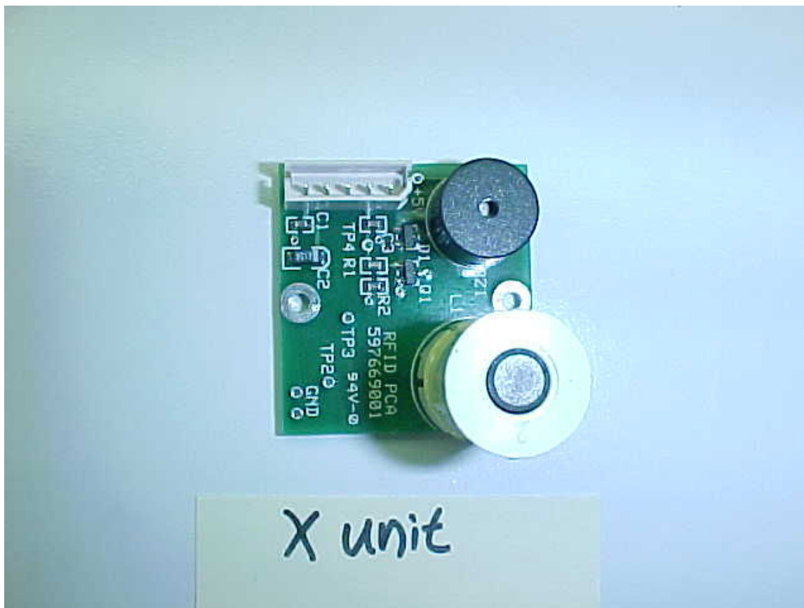
X unit Daughter PCB Board Layout.
