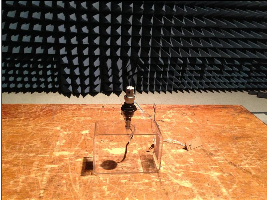
Photograph 6. Radiated Spurious Emissions, Test Setup, 1 GHz – 18 GHz, Setup
