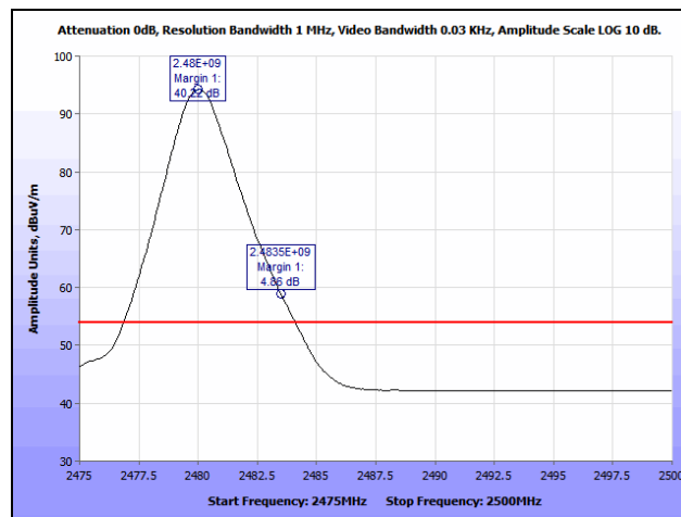
Plot 20. Radiated Restricted Band Edge, High Channel, Average In-Band
