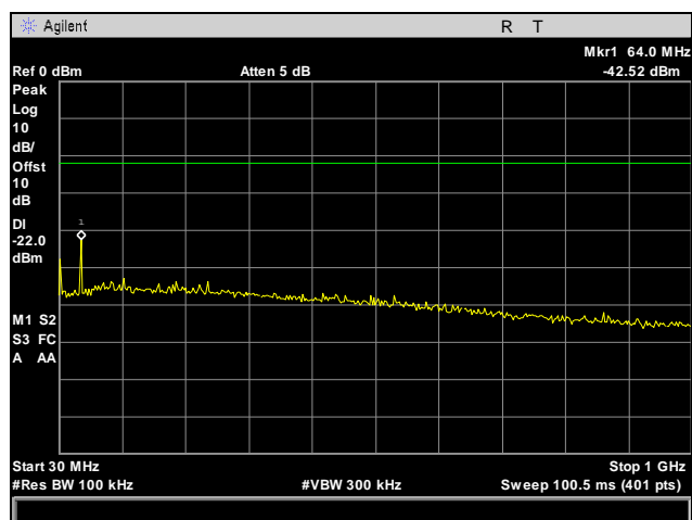
Plot 25. Conducted Spurious Emissions, Mid Channel, 30 MHz – 1 GHz
