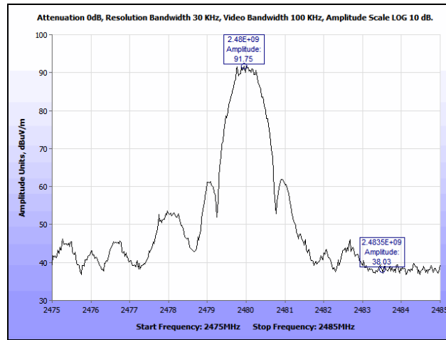
Plot 22. Radiated Restricted Band Edge, High Channel, Fundamental Delta
