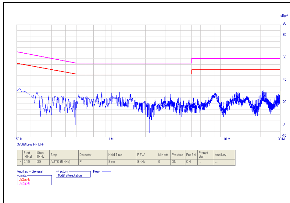
Plot 1. Conducted Emissions, Phase Line Plot
