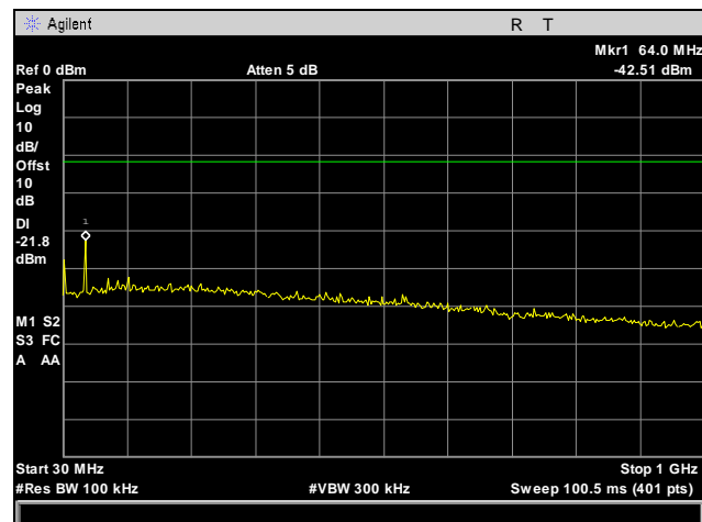
Plot 27. Conducted Spurious Emissions, High Channel, 30 MHz – 1 GHz
