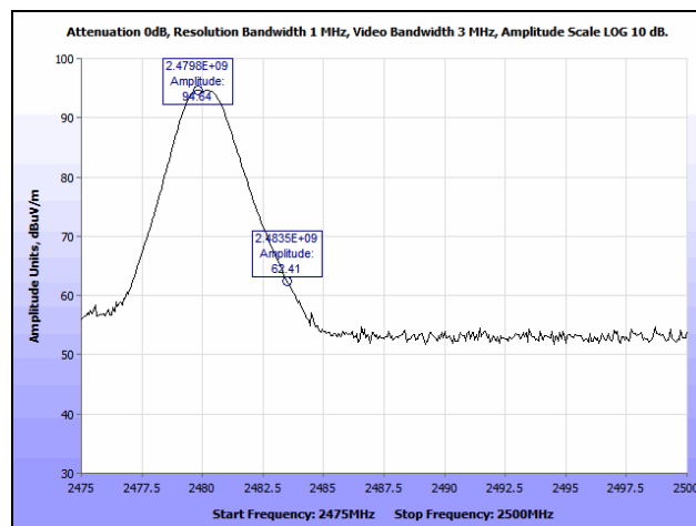
Plot 21. Radiated Restricted Band Edge, High Channel, Peak In-Band
