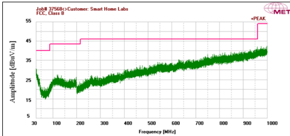
Plot 16. Radiated Spurious Emissions, High Channel, 30 MHz – 1 GHz
