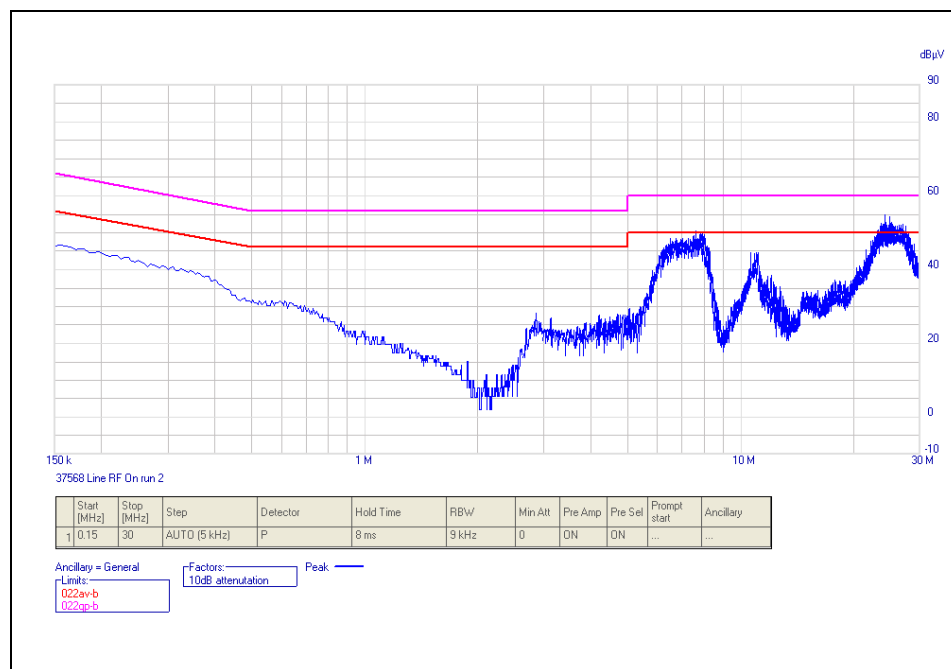
Plot 4. Conducted Emissions, 15.207(a), Phase Line
