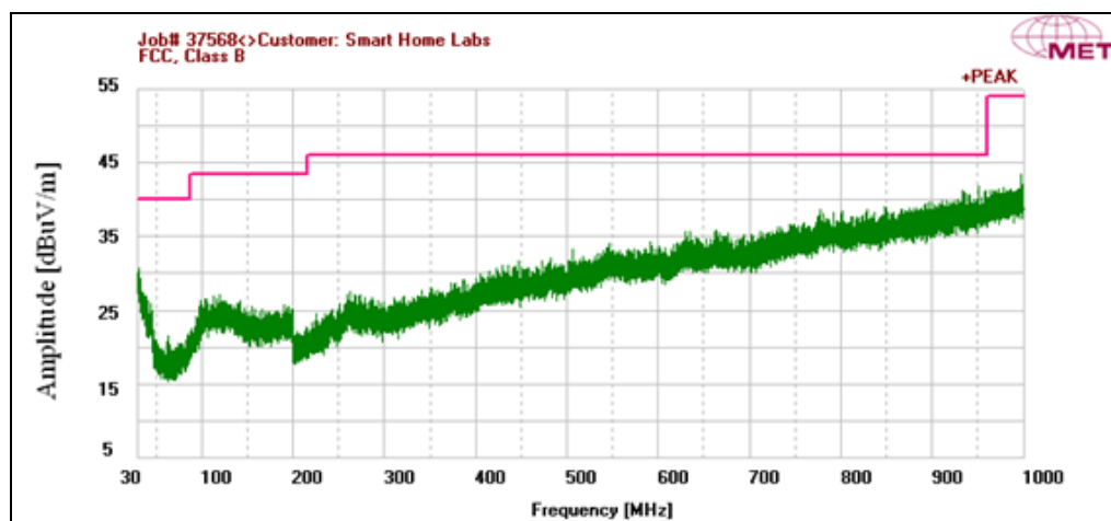
Plot 14. Radiated Spurious Emissions, Mid Channel, 30 MHz – 1 GHz
