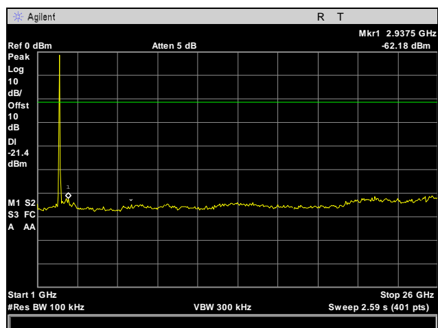
Plot 24. Conducted Spurious Emissions, Low Channel, 1 GHz – 26 GHz
