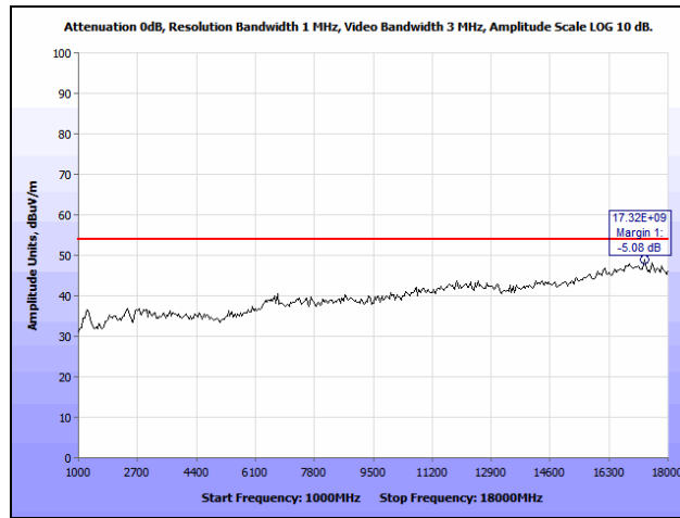
Plot 15. Radiated Spurious Emissions, Mid Channel, 1 GHz – 18 GHz
