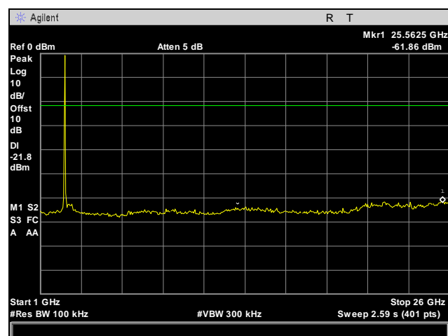
Plot 28. Conducted Spurious Emissions, High Channel, 1 GHz – 26 GHz
