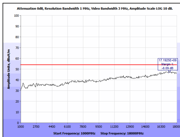
Plot 17. Radiated Spurious Emissions, High Channel, 1 GHz – 18 GHz
