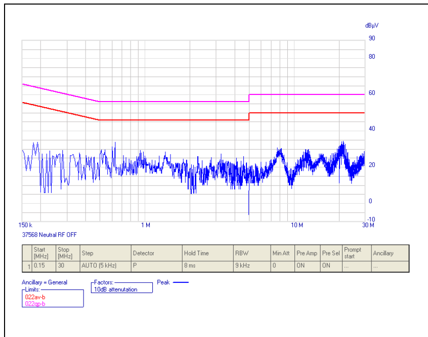
Plot 2. Conducted Emissions, Neutral Line Plot
