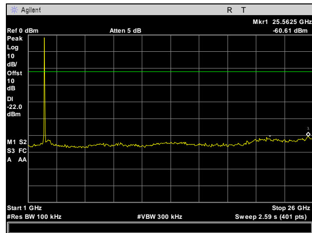
Plot 26. Conducted Spurious Emissions, Mid Channel, 1 GHz – 26 GHz
