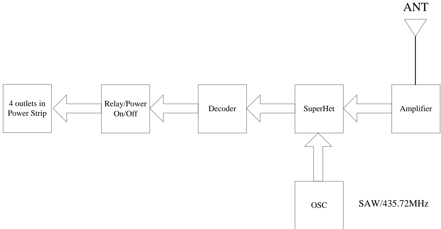
Block diagram of Receiver
