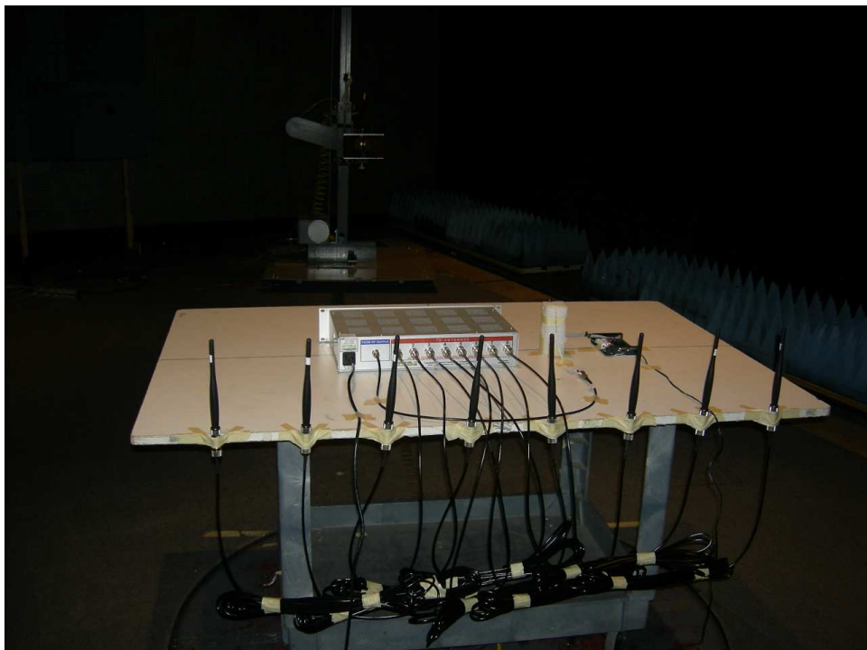
Figure 6: Radiated Emissions – Whip Antenna – YPOS
