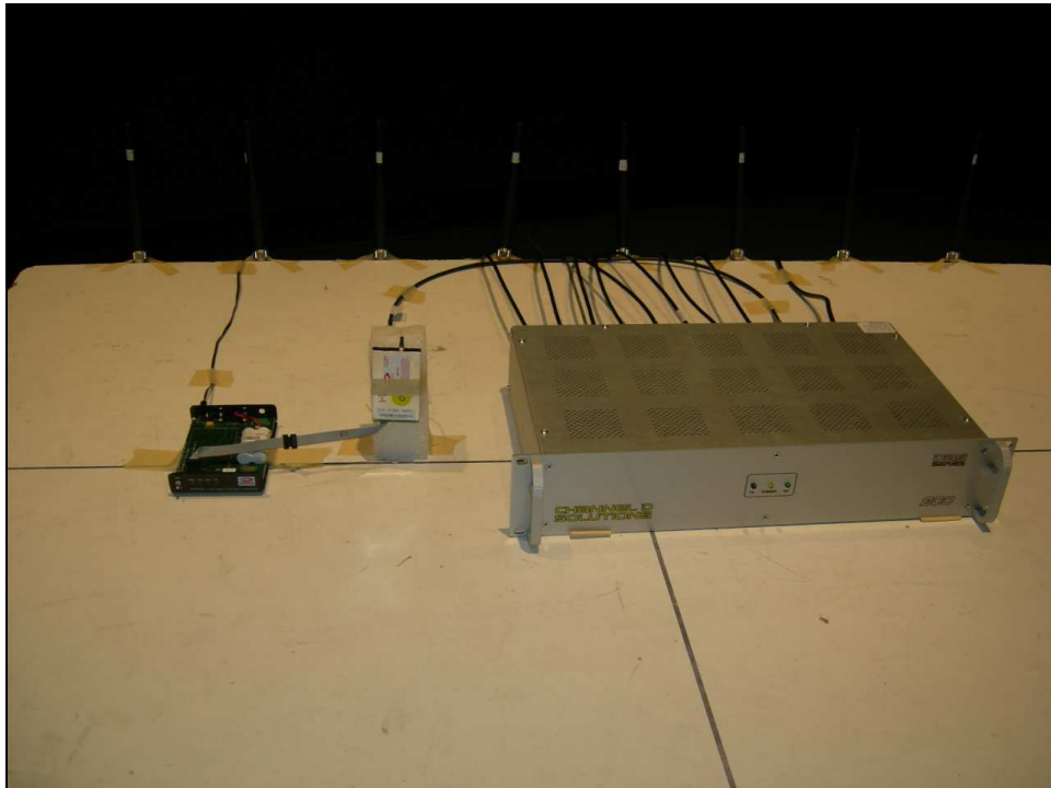
Figure 5: Radiated Emissions – Whip Antenna – YPOS
