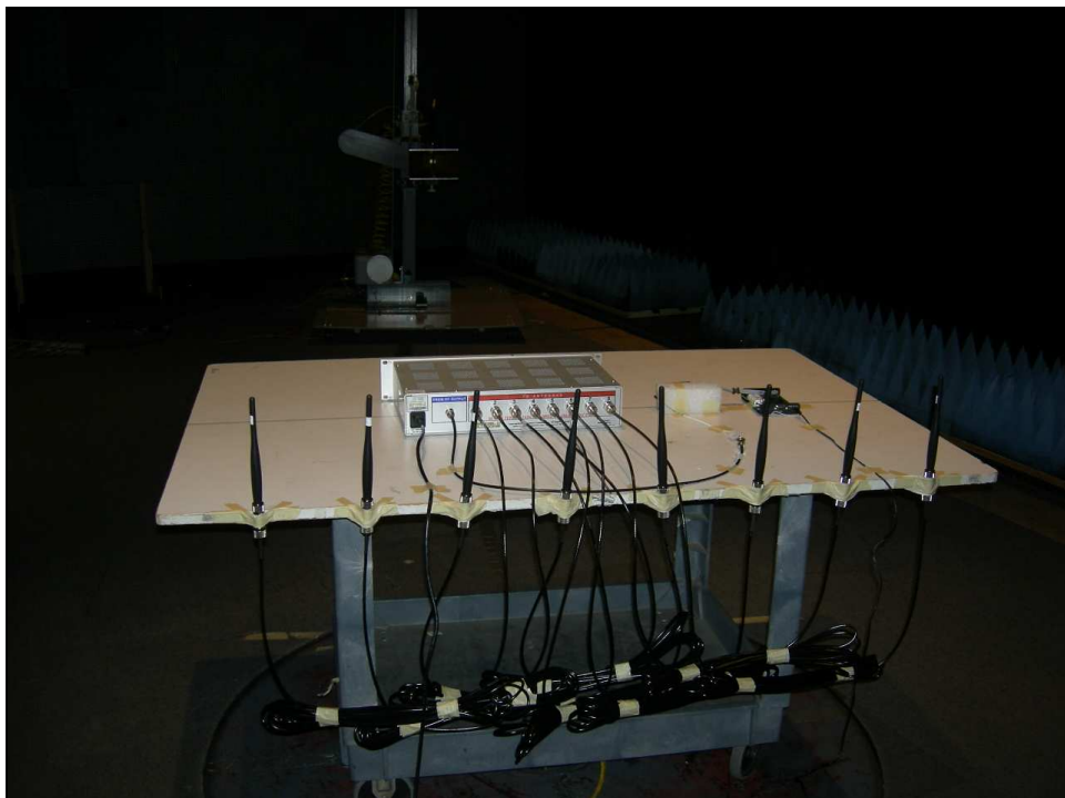
Figure 8: Radiated Emissions – Whip Antenna – ZPOS
