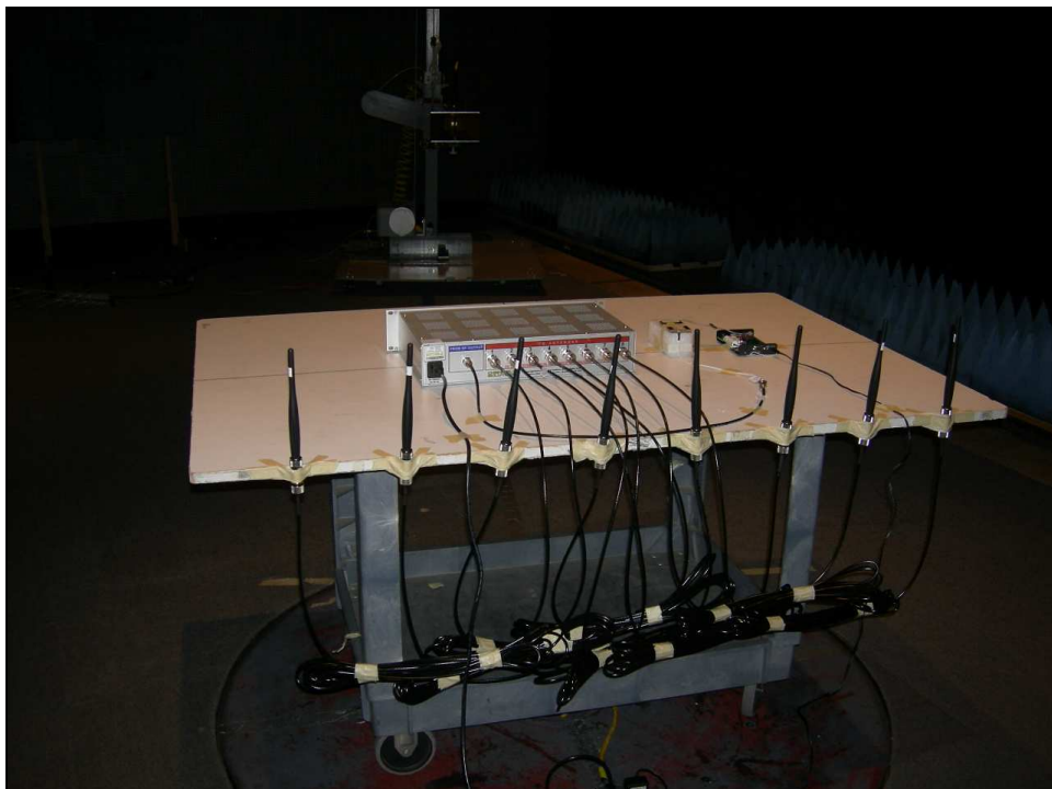
Figure 4: Radiated Emissions – Whip Antenna – XPOS
