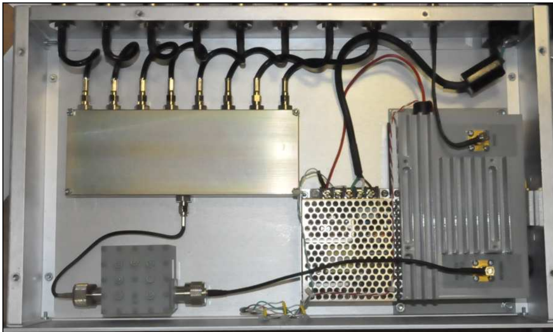
Figure 3: Amplifier
