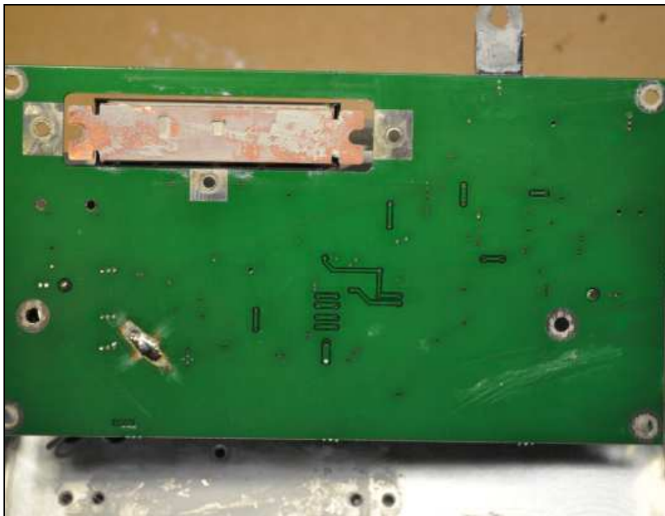
Figure 5: Amplifier PCB
