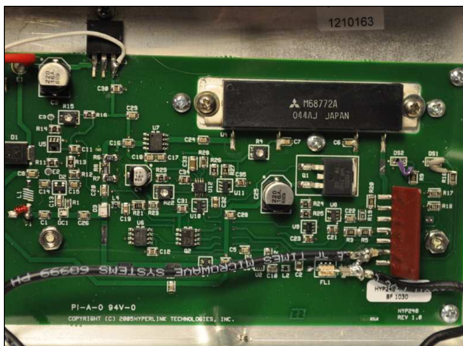
Figure 4: Amplifier PCB
