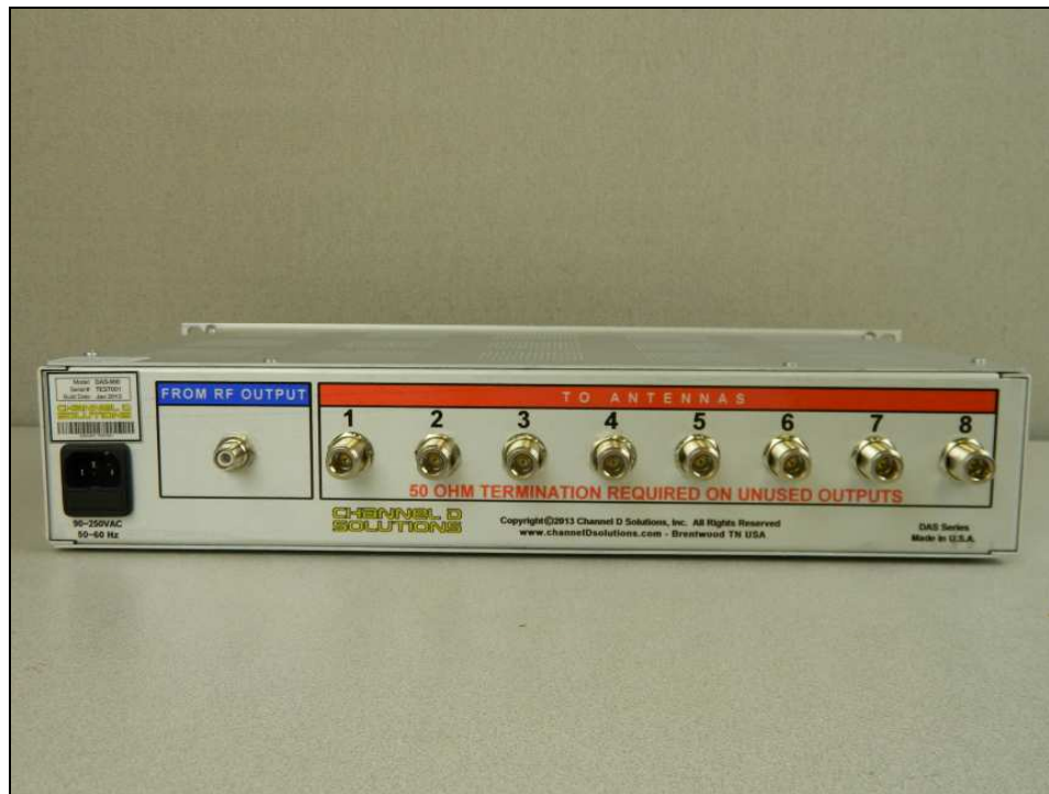
Figure 7: Amplifier
