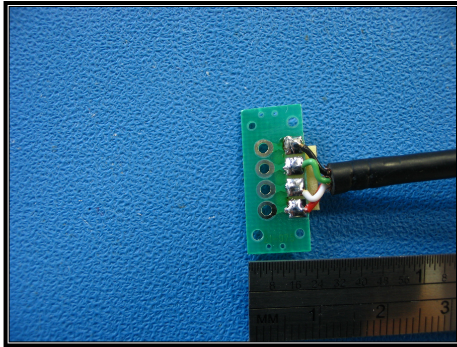
PHOTOGRAPH 16: USB CABLE PCB
