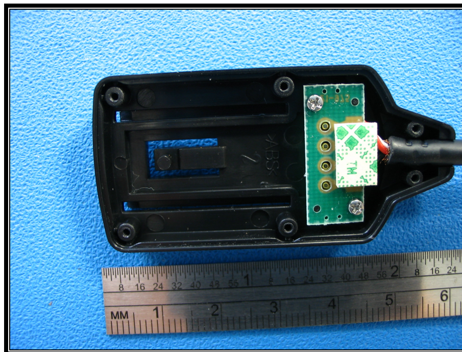
PHOTOGRAPH 15: USB CABLE INSIDE VIEW
