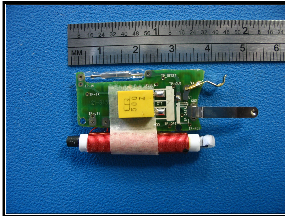
PHOTOGRAPH 12: TRANSMITTER PCB BACK VIEW
