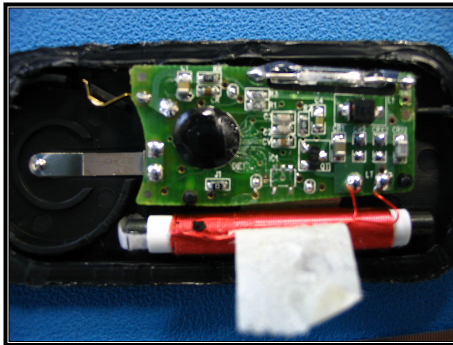
PHOTOGRAPH 11: FRONT OF TRANSMITTER CIRCUIT BOARD IN HOUSING WITH TAPE LIFTED
