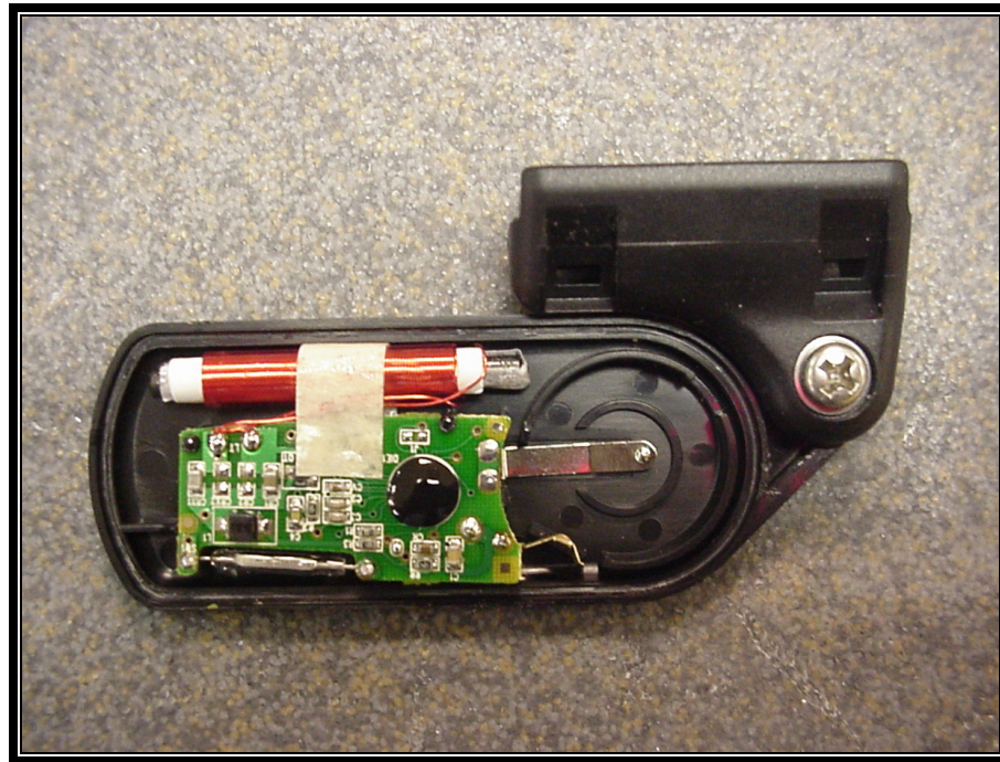
PHOTOGRAPH 10: FRONT OF TRANSMITTER CIRCUIT BOARD IN HOUSING
