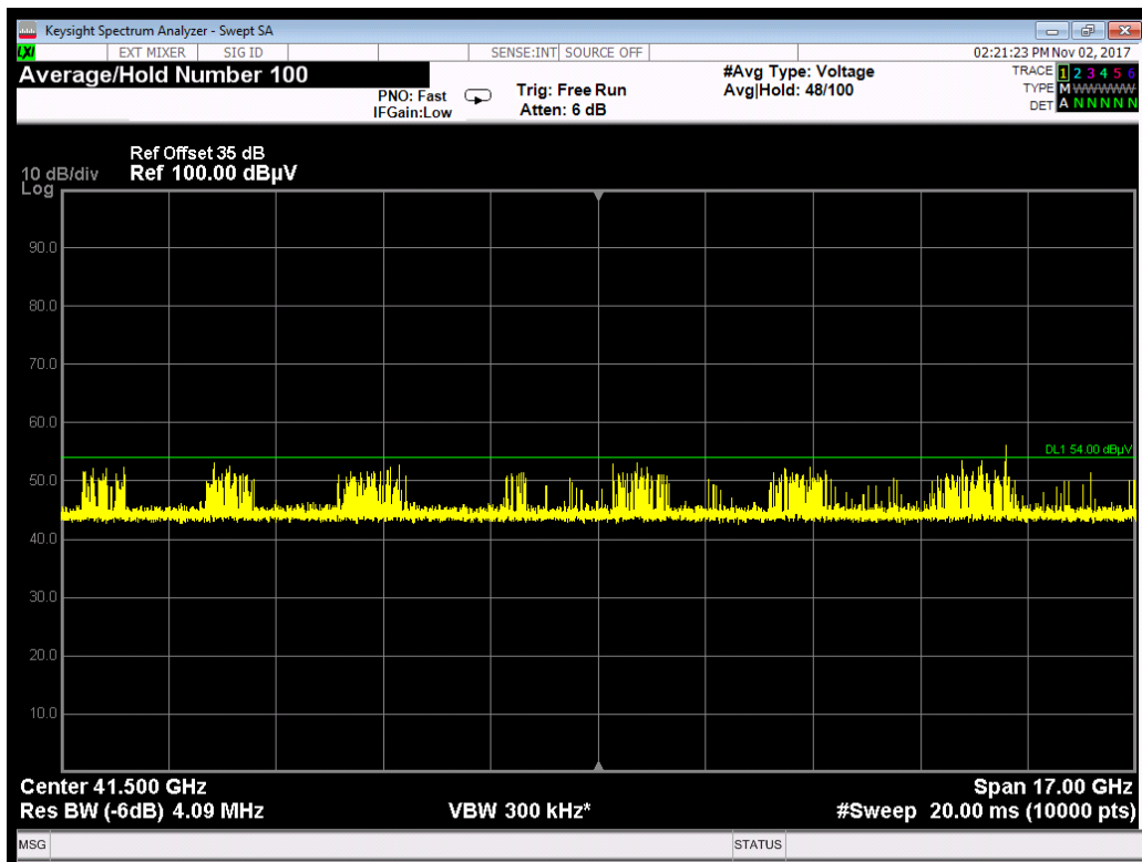
33 – 50 GHz : Average Detector Plot
