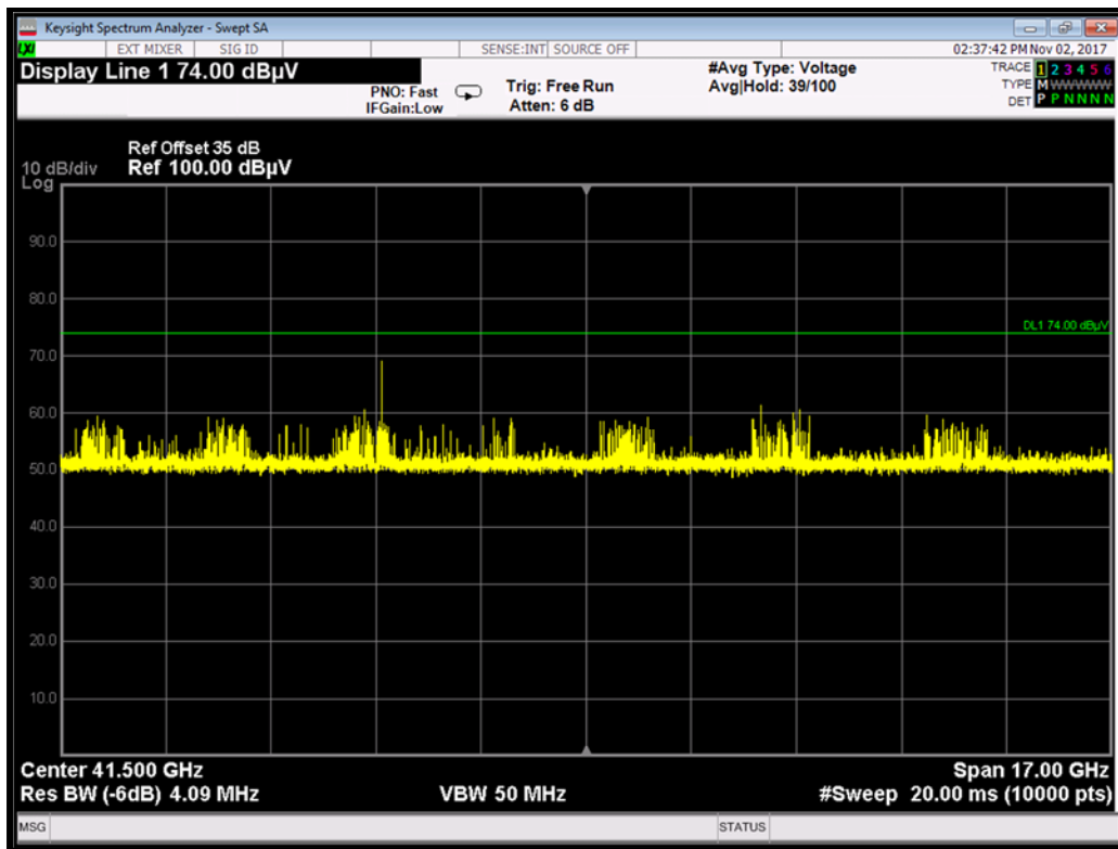
33 – 50 GHz : Peak Detector Plot
