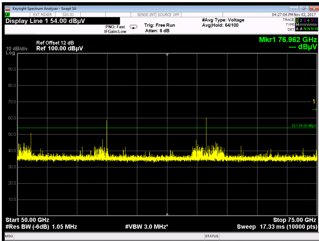
50 – 75 GHz : Average Detector Plot
