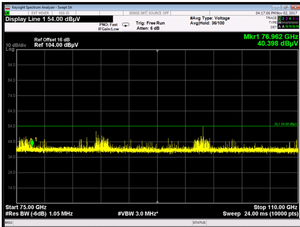
75- 110 GHz : Average Detector Plot
