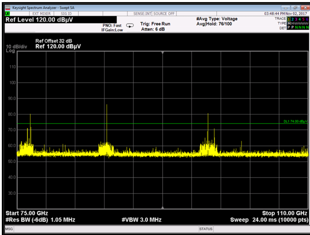
75 – 110 GHz : Peak Detector Plot
