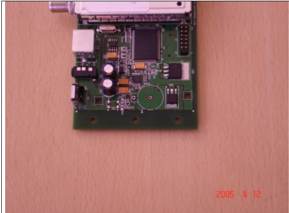
Partial view on component side
