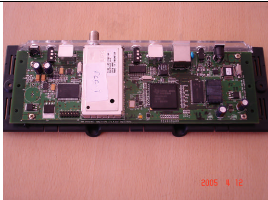
Over view without top enclosure
