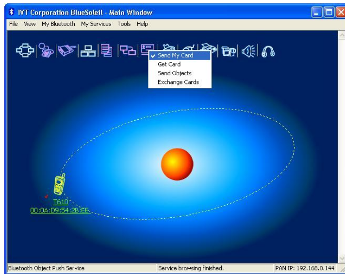
Figure 3.6: Send Object
