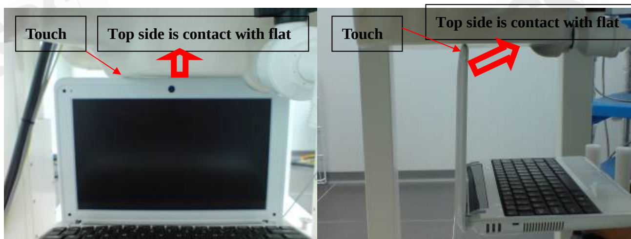
Fig.4 Top side of Notebook is paralleled flat phantom, open the panel with 90 degrees , top side is contact with flat phantom.
