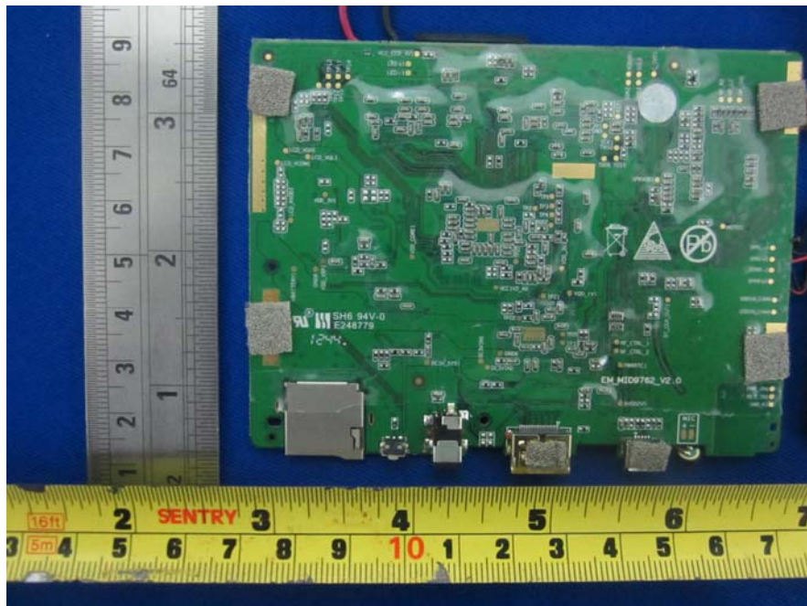
EUT – Main Board Bottom with Conductive Foam View
