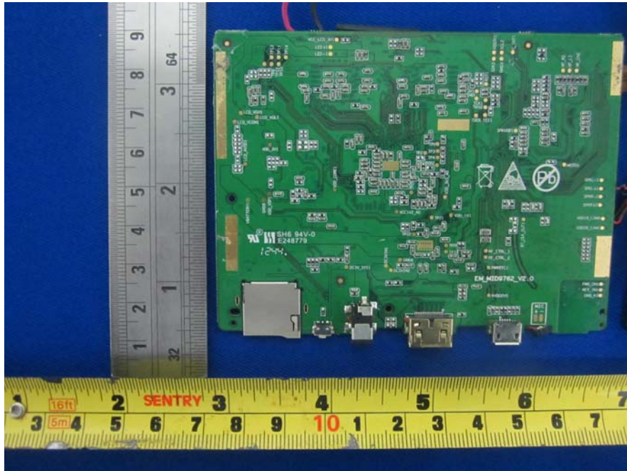
EUT –Main Board Bottom without Conductive Foam View
