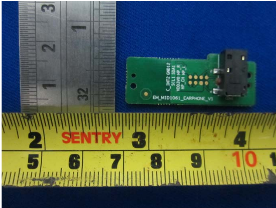
EUT –Earphone Board Bottom View
