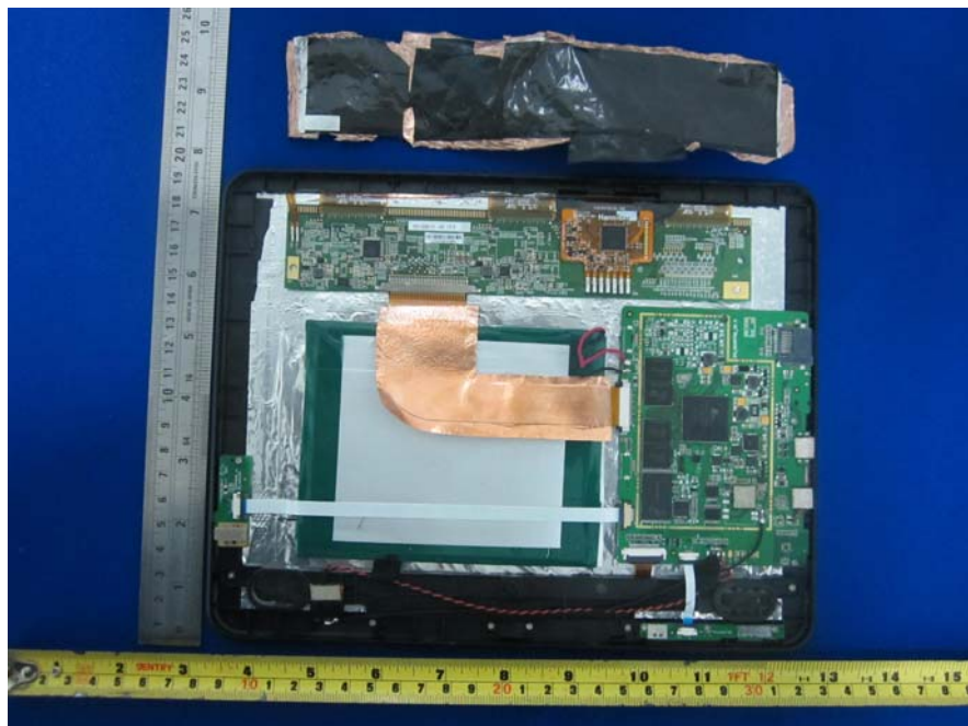
EUT –Copper Foil Cover off View
