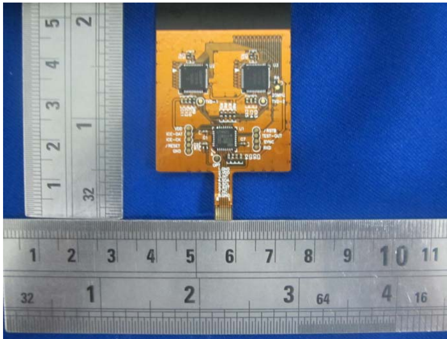
EUT – Touch Plan Board Top View
