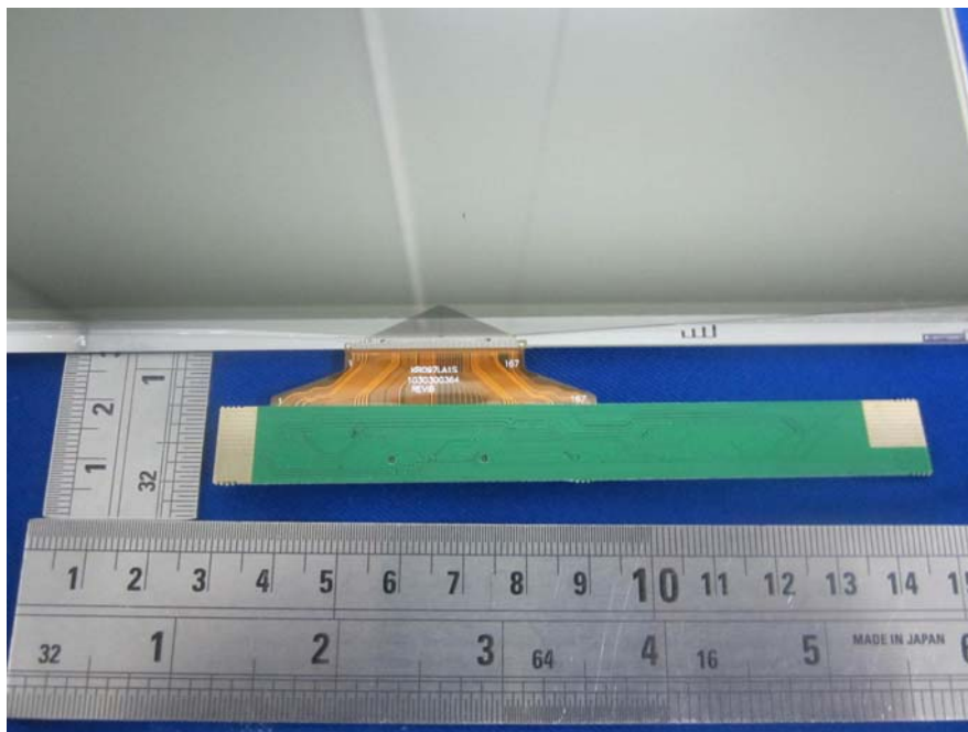
EUT –LED Display control Board Bottom View
