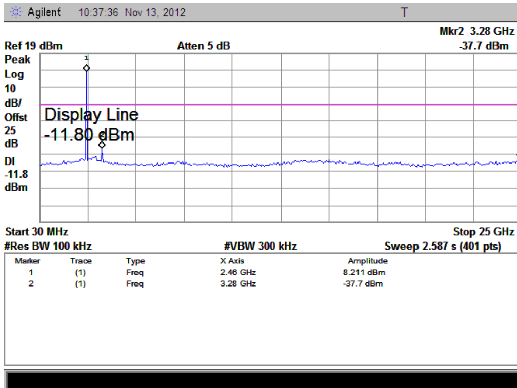
(Plot H.1: Channel = 39, 30MHz to 25GHz)
