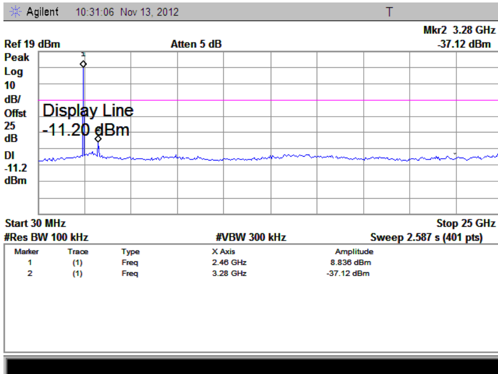
(Plot E.1: Channel = 39, 30MHz to 25GHz)
