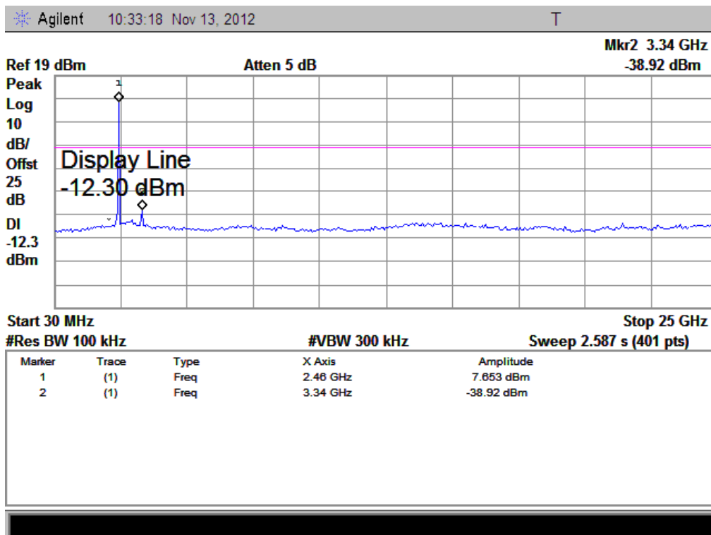
(Plot F.1: Channel = 78, 30MHz to 25GHz)
