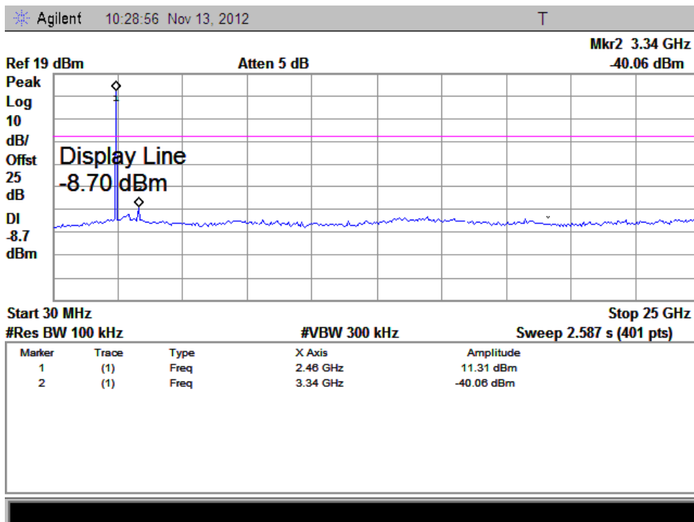
(Plot C.1: Channel = 78, 30MHz to 25GHz)
