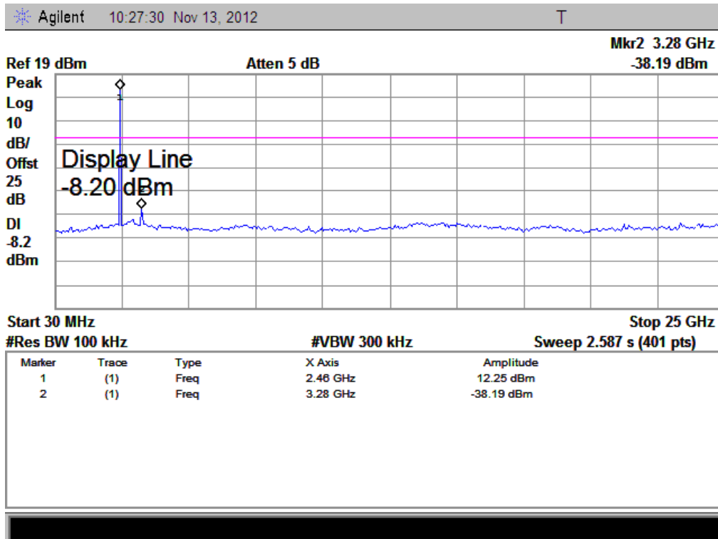
(Plot B.1: Channel = 39, 30MHz to 25GHz)
