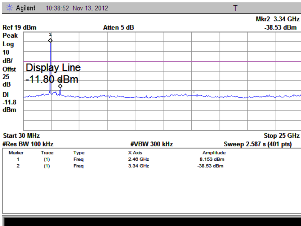
(Plot I.1: Channel = 78, 30MHz to 25GHz)
