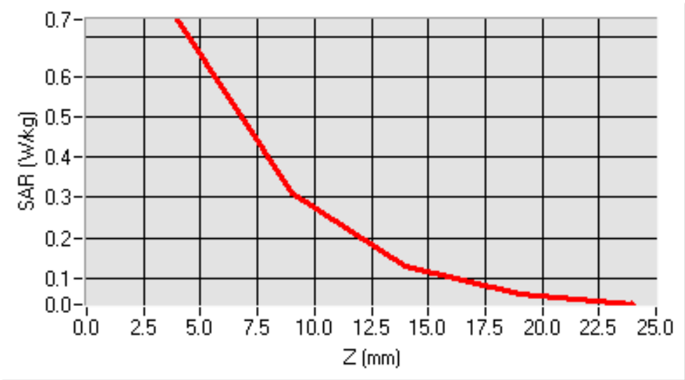
SAR, Z Axis Scan (X = -3, Y = -7)
