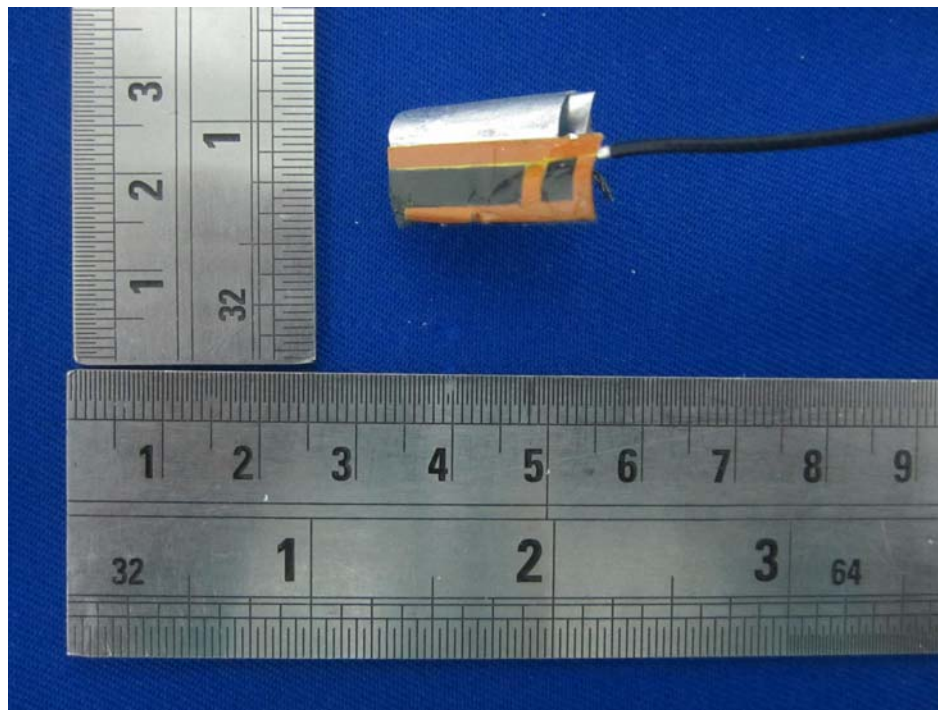
EUT – Loudspeake View
