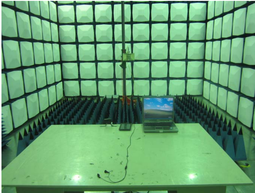
Radiated Emission above 1G-Rear View
