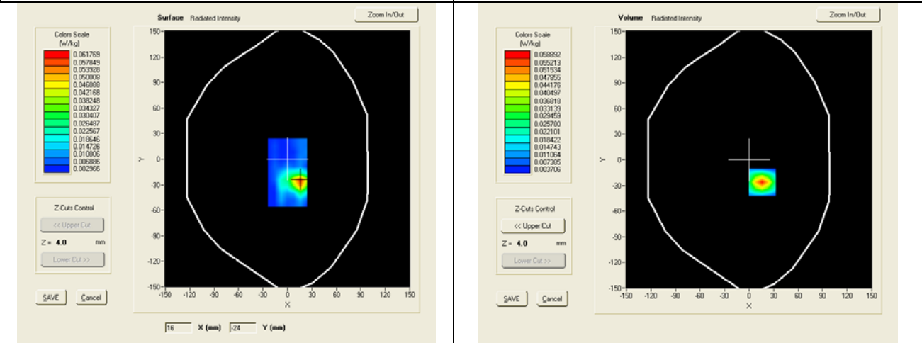
SAR, Z Axis Scan (X = 16, Y = -26)
