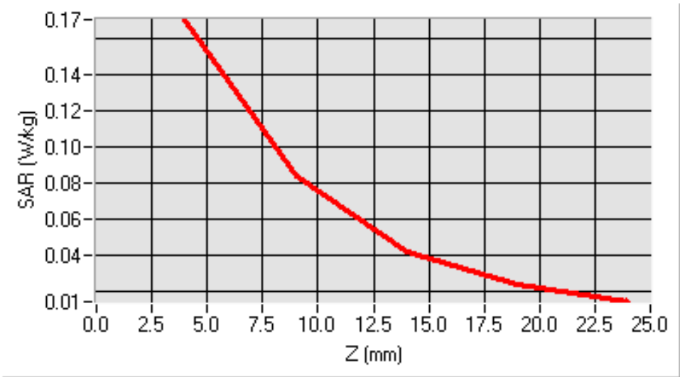
SAR, Z Axis Scan (X = 16, Y = 23)
