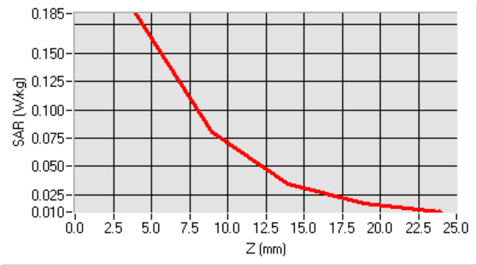
SAR, Z Axis Scan (X = 16, Y = 21)
