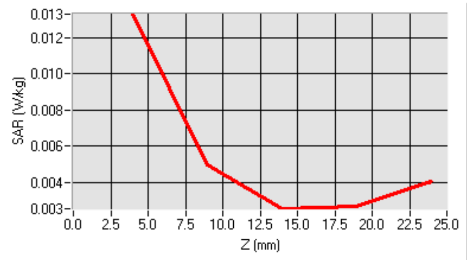
SAR, Z Axis Scan (X = -8, Y = 15)
