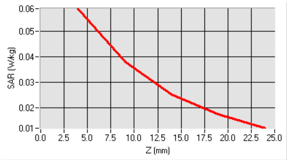
SAR, Z Axis Scan (X = 16, Y = -26)
