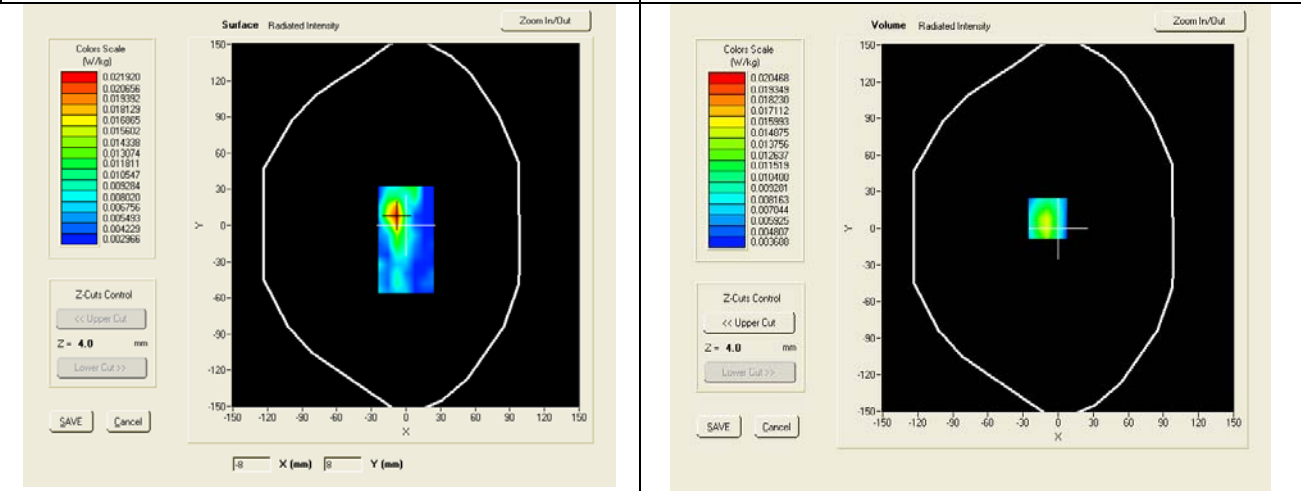
SAR, Z Axis Scan (X = -9, Y = 8)
