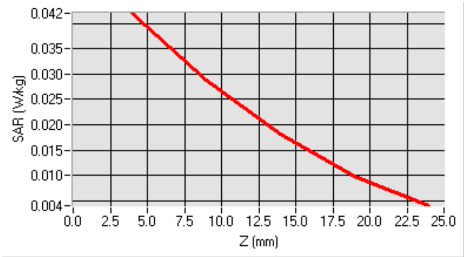
SAR, Z Axis Scan (X = 19, Y = -25)
