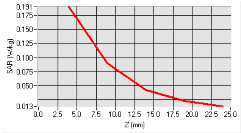
SAR, Z Axis Scan (X = 15, Y = 21)
