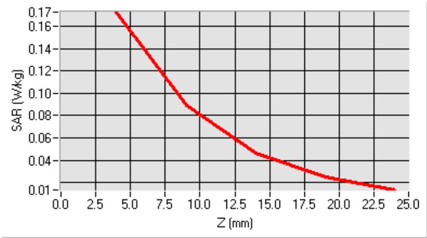
SAR, Z Axis Scan (X = 16, Y = 23)
