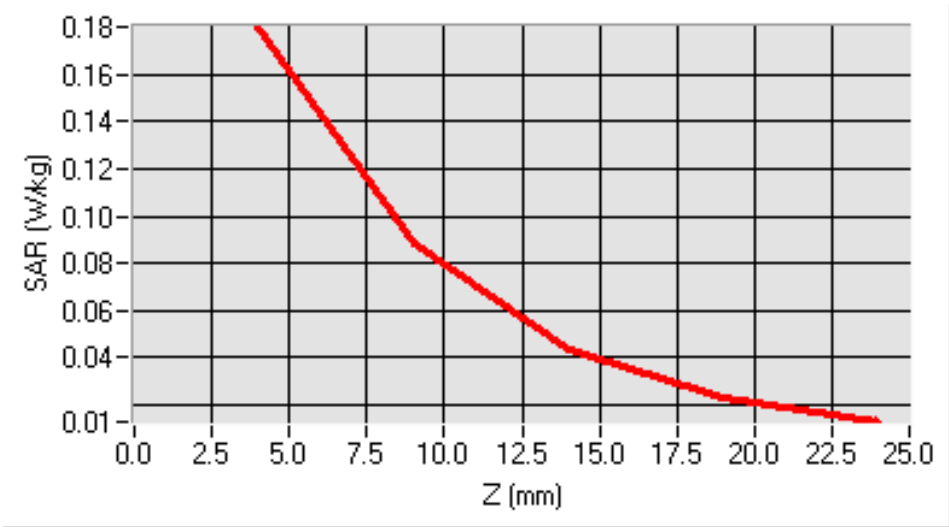
SAR, Z Axis Scan (X = 15, Y = 22)
