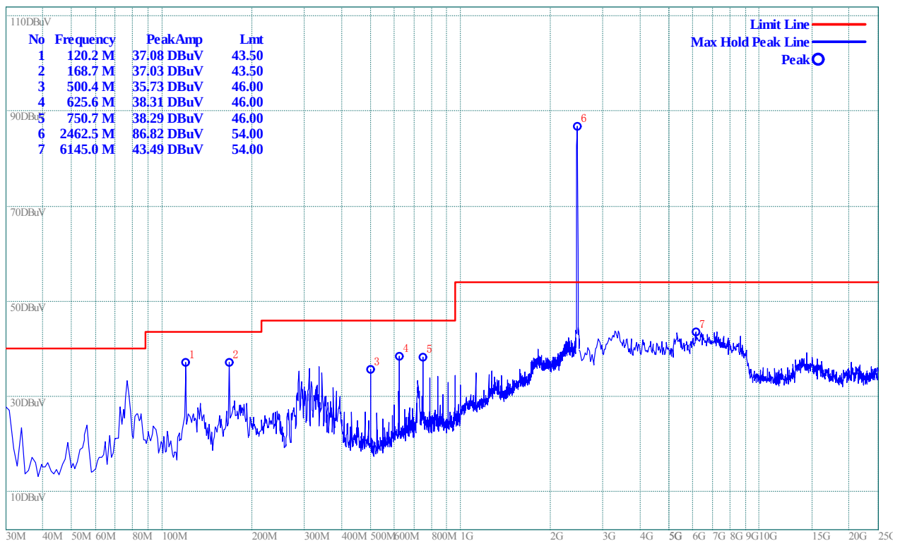
(Plot F.2: Antenna Horizontal, 30MHz to 25GHz)
