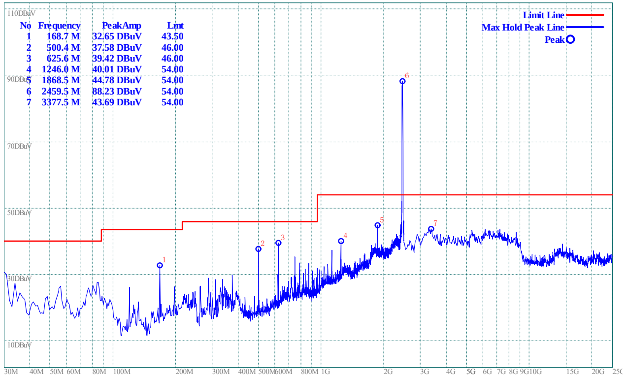
(Plot F.3: Antenna Vertical, 30MHz to 25GHz)
