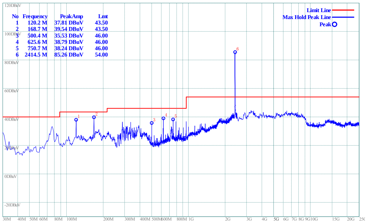
(Plot D.2: Antenna Horizontal, 30MHz to 25GHz)
