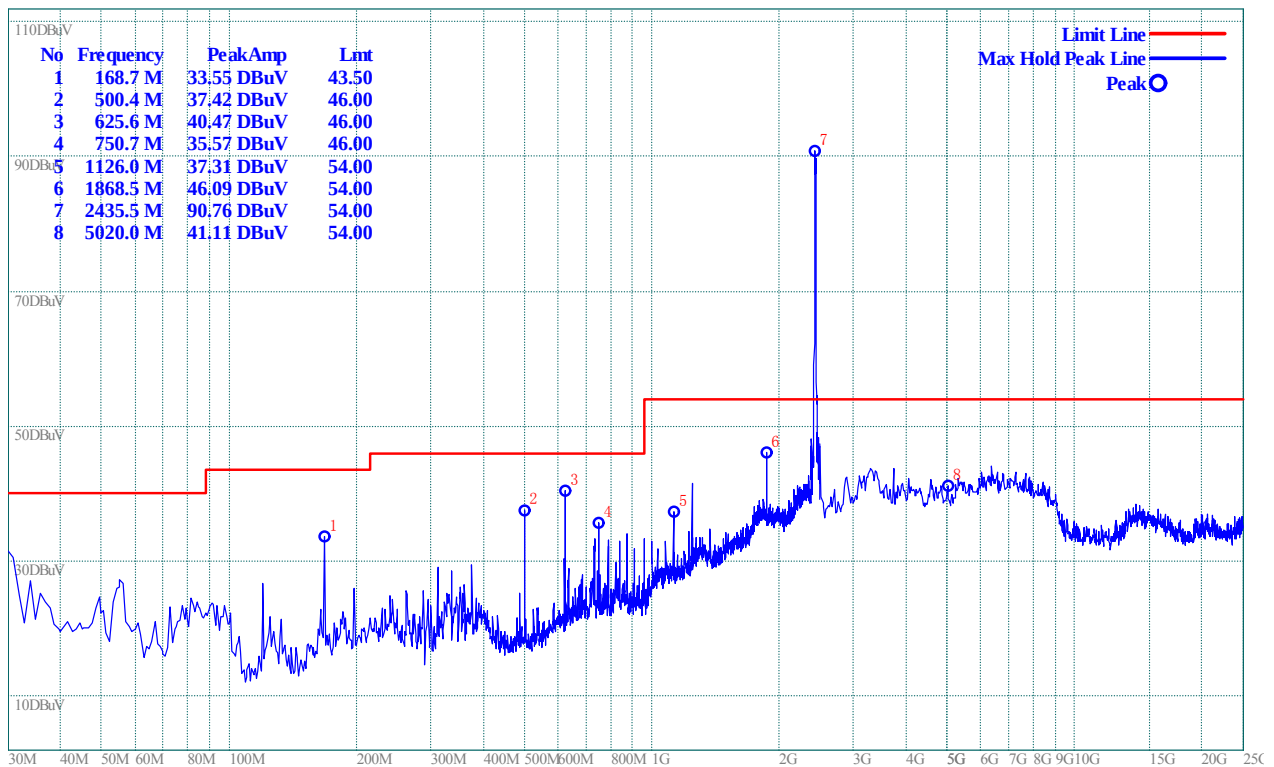
(Plot E.3: Antenna Vertical, 30MHz to 25GHz)
