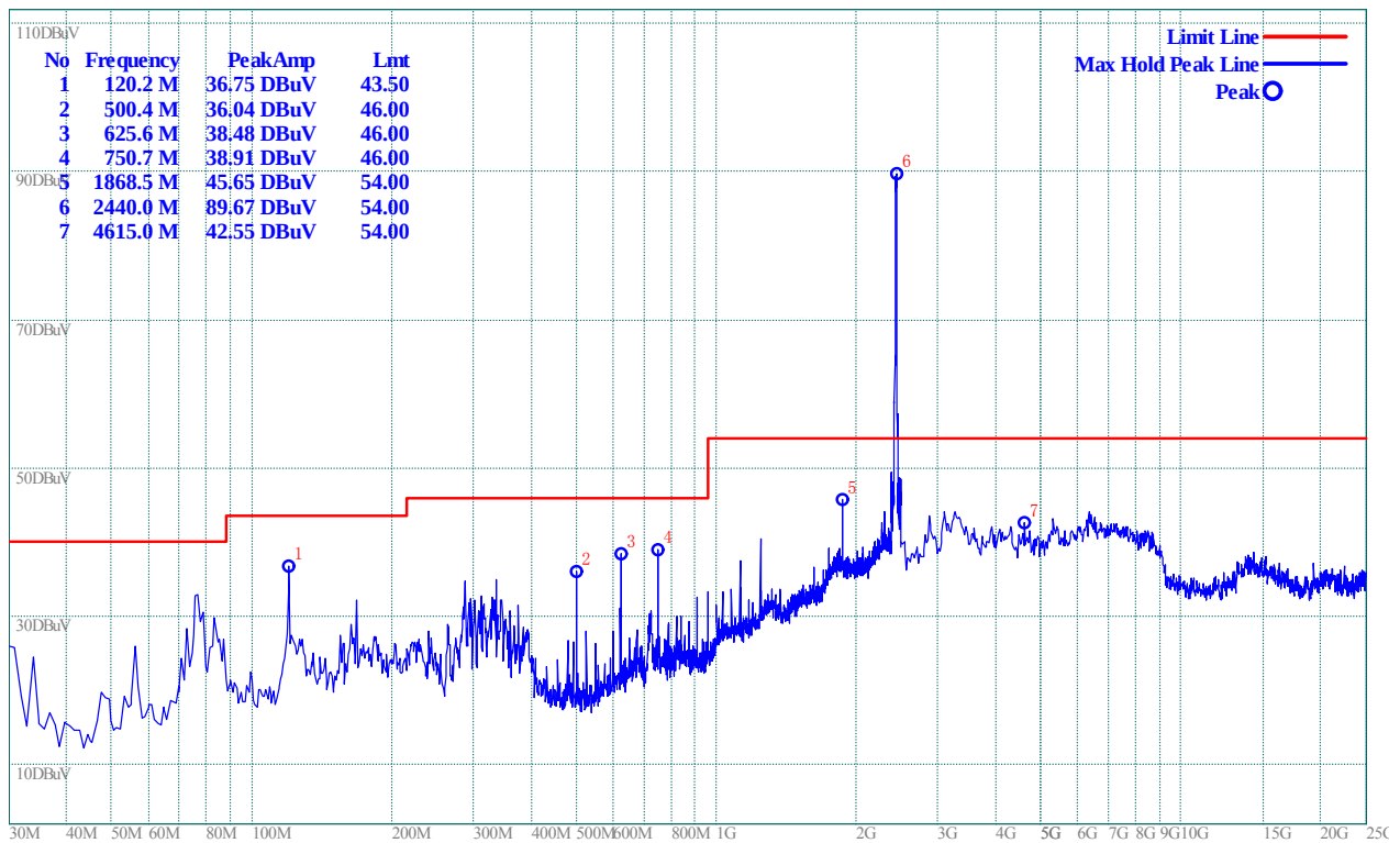
(Plot E.2: Antenna Horizontal, 30MHz to 25GHz)
