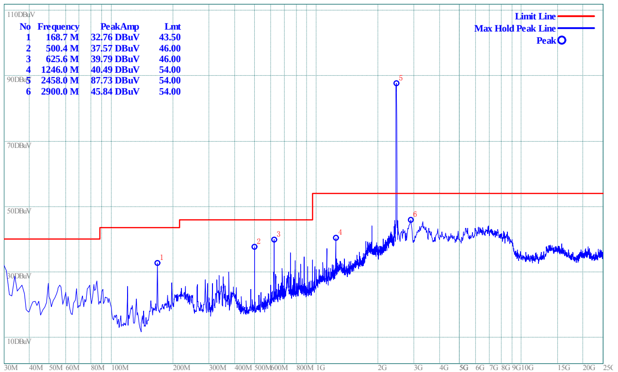
(Plot I.3: Antenna Vertical, 30MHz to 25GHz)
