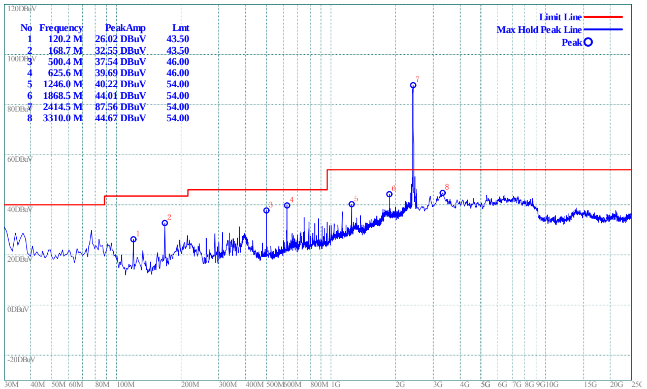
(Plot D.3: Antenna Vertical, 30MHz to 25GHz)
