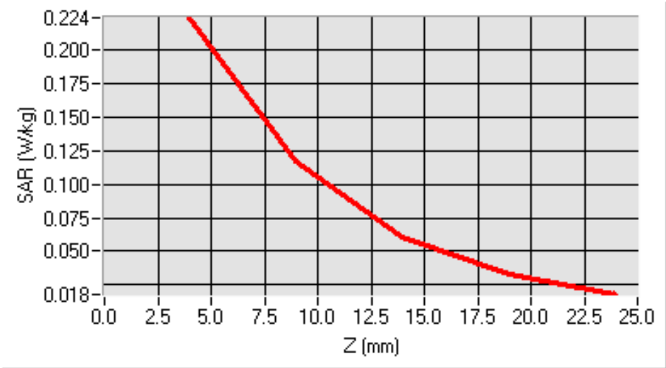
SAR, Z Axis Scan (X = -5, Y = -16)
