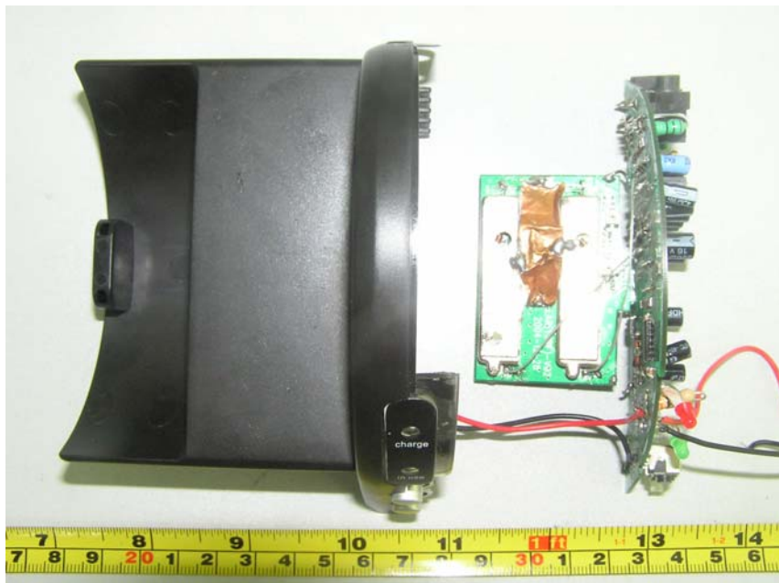
EUT- Inside View (4)
