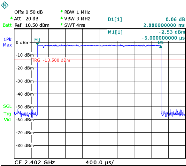
Pi/4DQPSK DH5 Low Channel
