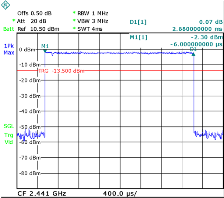
Pi/4DQPSK DH5 Middle Channel
