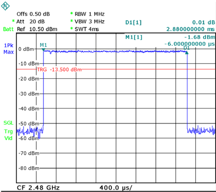
Pi/4DQPSK DH5 High Channel
