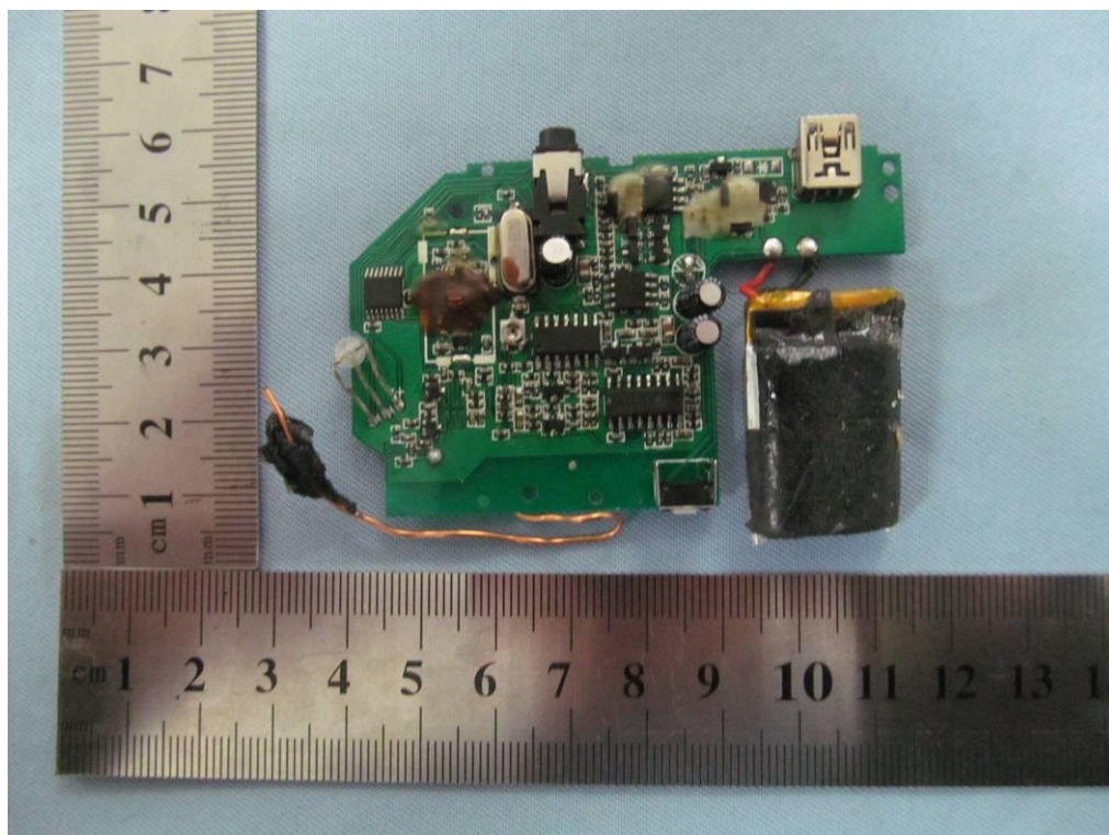
INTERNAL VIEW-1 OF ET
