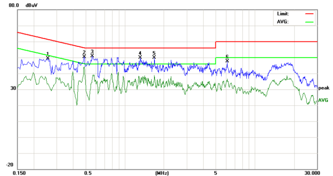
Line Conducted Emission Test Line 2-N
