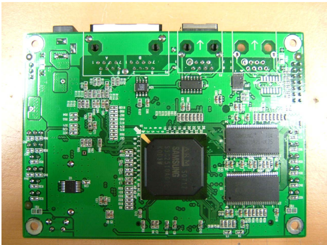
PS110W Rear Board Photo
