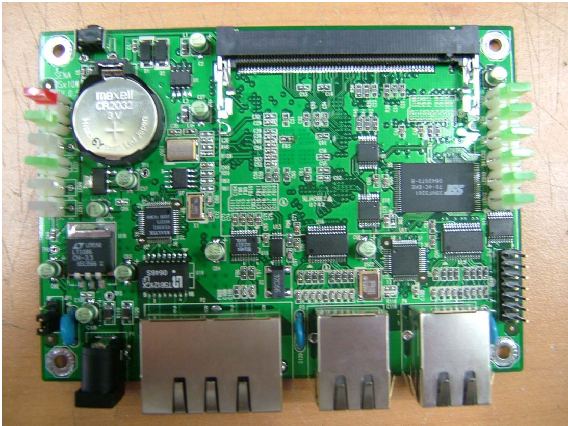
PS210W Rear Board Photo
