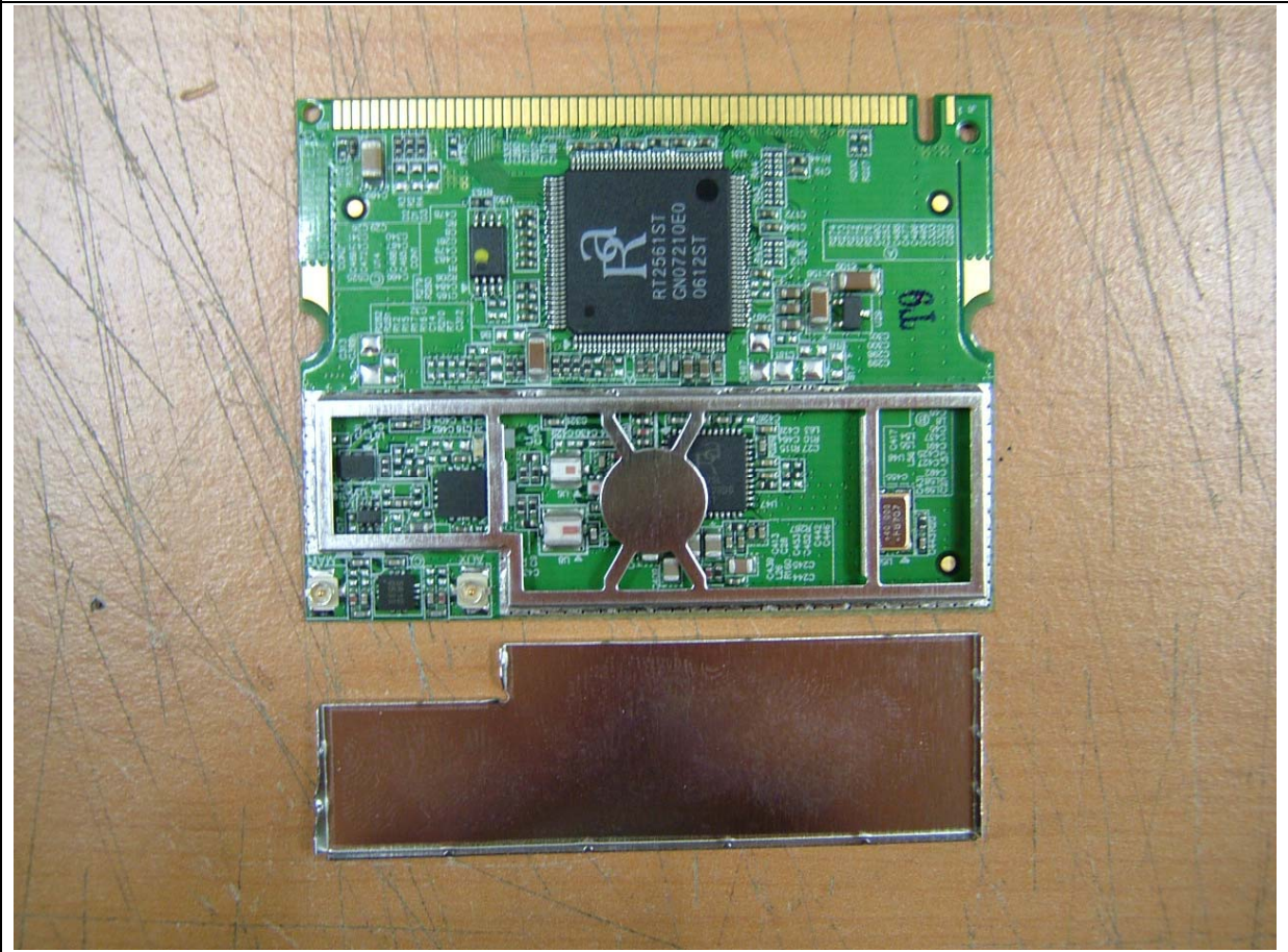
WLAN Inside Board Photo
