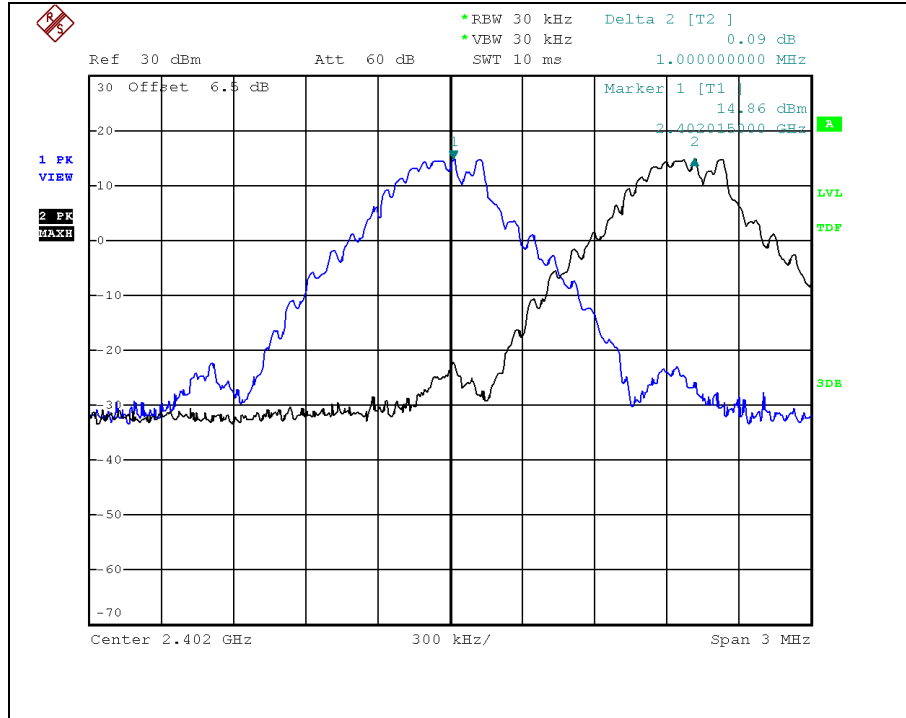
GFSK _ Low frequency
