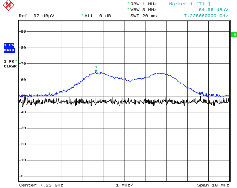
Radiated Spurious Emissions plot – Peak Reading (CH.12 3rd Harmonic)
