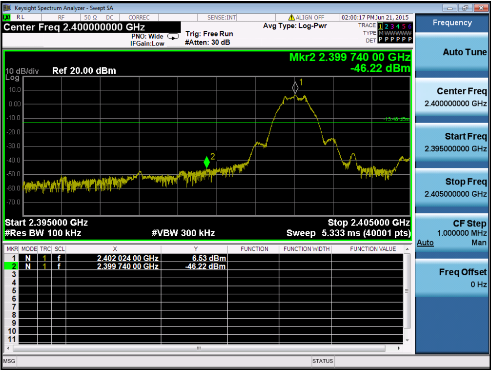
Low Band-edge (Test Frequency : 2402 MHz)
