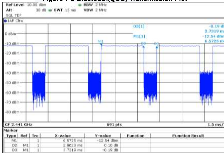
Figure 7-2 Bluetooth(QCC) Transmission Plot
