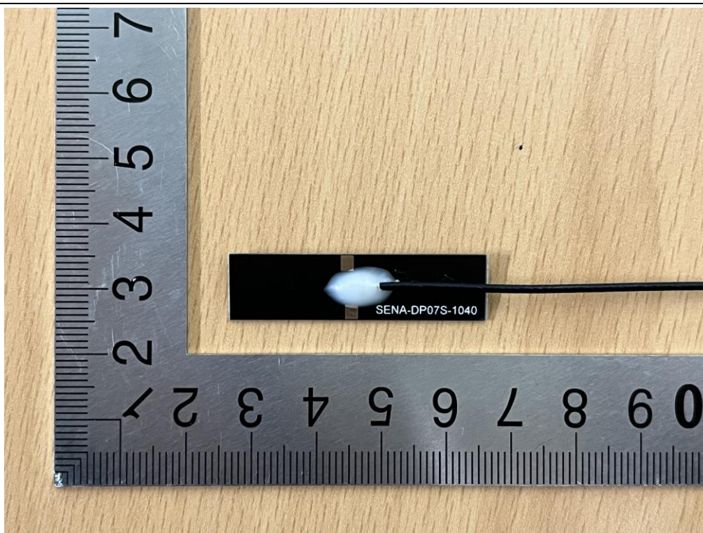
MESH Antenna Type1(Antenna cable length: 20 cm)
