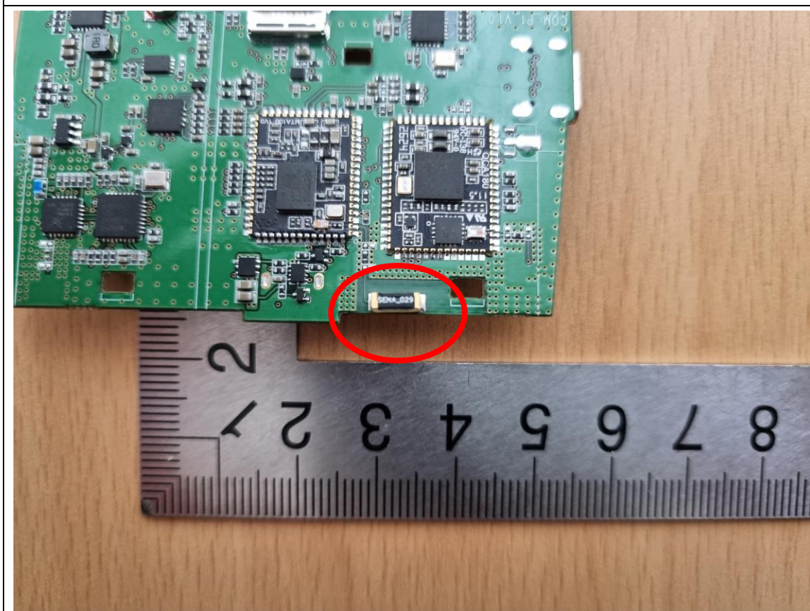
BT2 Antenna
