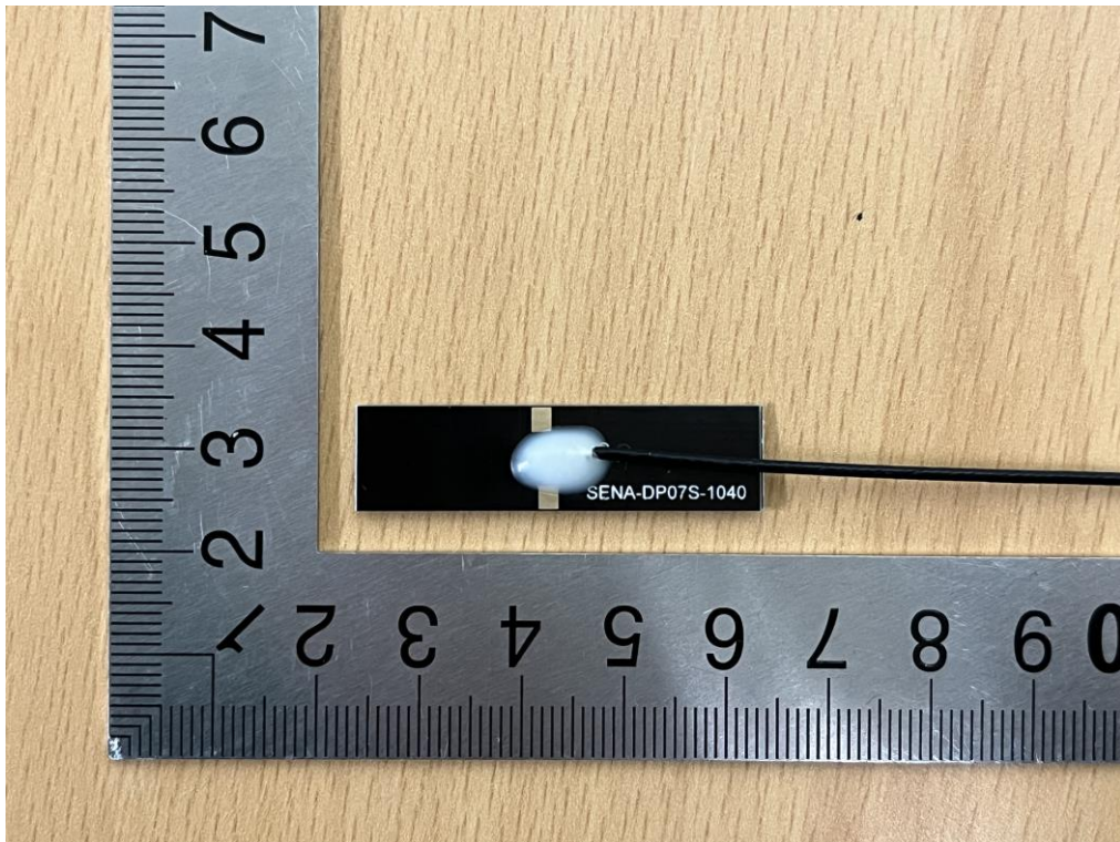
BT1 Antenna
