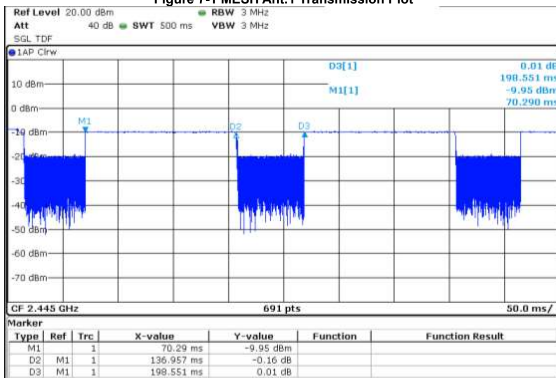
Figure 7-1 MESH Ant.1 Transmission Plot
